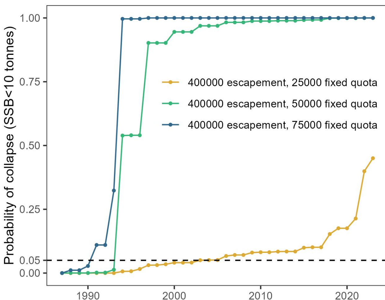
Figure 2: Annual proportions of iterations when 1 April SSB collapsed for a Bescapement=400,000 tonnes and different fixed minimum quotas. Collapse is defined as SSB dropping below 10 tonnes (i.e. effectively zero) and not recovering in the subsequent period. Proportions are computed over 2,779 iterations.
