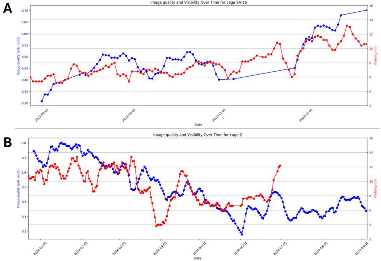
Figure 10. An average measure of image quality (arbitrary units) from the underwater camera at the small scale site (A), and Cage 2 from the large scale site (B), compared with Secchi disk measurements of visibility (m) at the small scale trial location.
