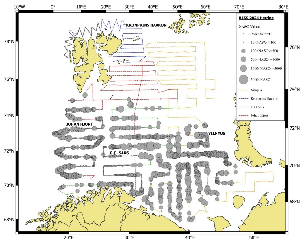
Figure 7.3.1.1 Geographical distribution of herring in autumn 2024 based on acoustic recordings. Circle sizes correspond to NASC values ( m^2/nm^2 ) per nautical mile.
