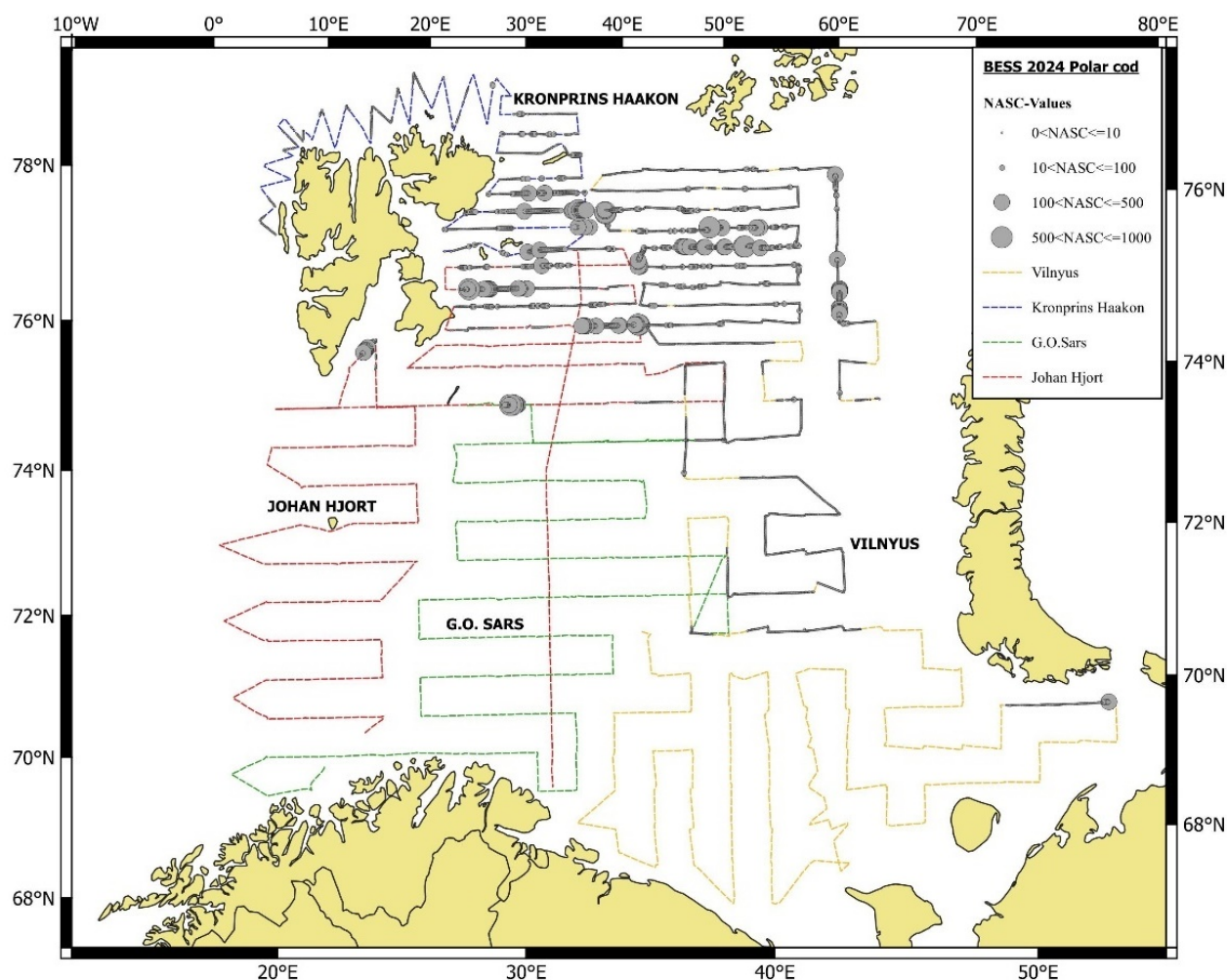
Figure 7.2.1.1 Geographical distribution of polar cod in autumn 2024 based on acoustic data. Circle sizes correspond to NASC values ( m^2/nmi^2 ) per nautical mile.
