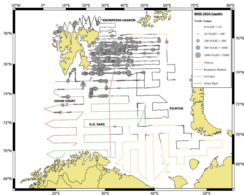
Figure. 7.1.1.1 Geographical distribution of capelin in autumn 2024 based on acoustic recordings. Circle sizes correspond to NASC values ( \text{m}^2/\text{nmi}^2 ) per nautical mile.
