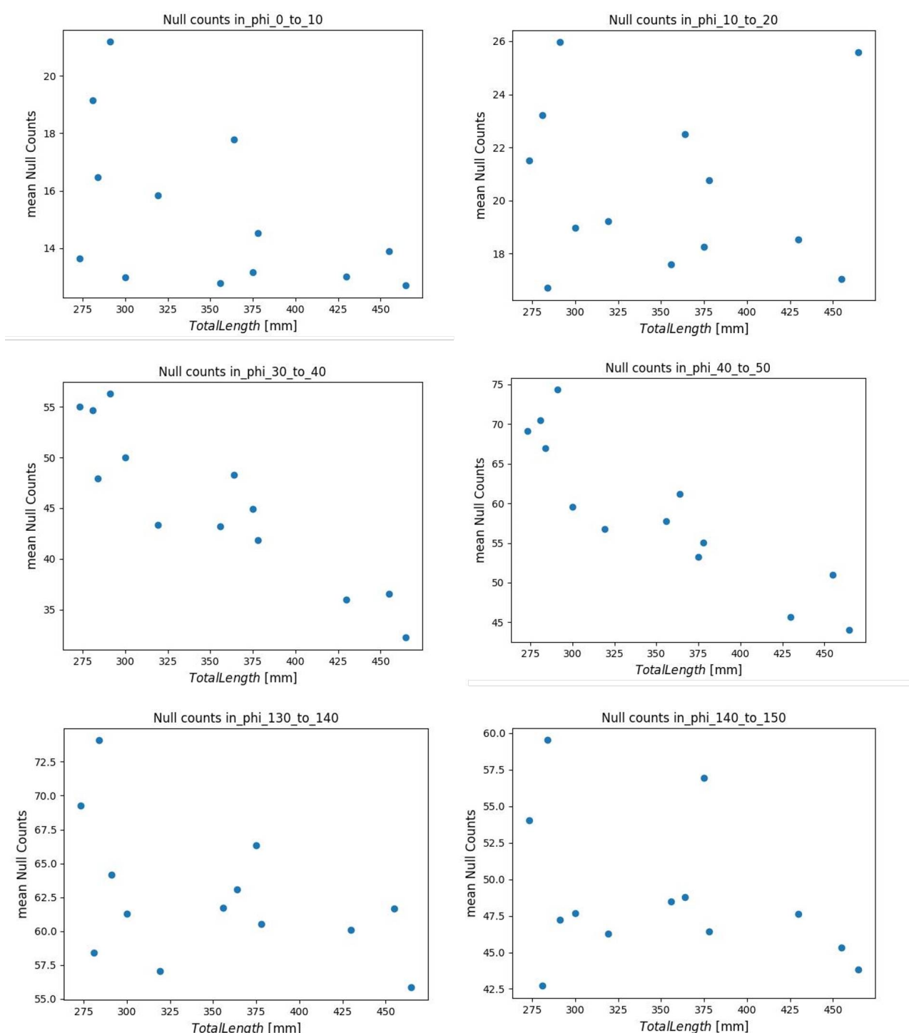
Figure 22. Average number of detected nulls in the measured TS frequency response within 10-degree tilt angles as a function of fish length. A clear correlation is not observed between the number of nulls and fish size. Even though, for tilt angles within 30–40° and 40–50°, there is a correlation, the number of nulls decreases as fish length increases, which is the opposite of expected.
