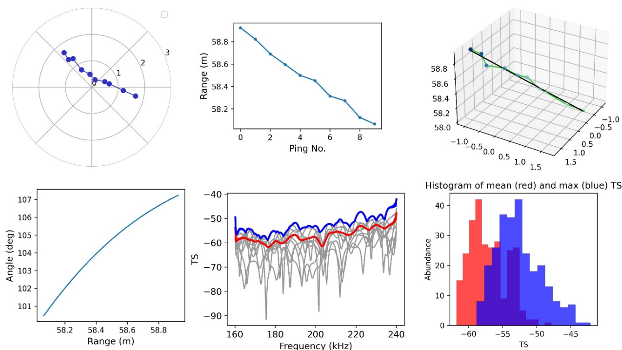
Figure 8. The location of target in the beam is estimated from athwartship and alongship angles. The target range to the transducer for different pings is estimated by split-beam echosounder. Spatial track of the target is estimated using Equation ( 3) . The estimated angle between the fish track and the acoustic axis of the transducer is plotted at different ranges. Measured target strength (TS) frequency response at of different pings together with the mean (red) and maximum (blue) TS as a function of frequency are shown. The histogram of the mean and maximum TS frequency responses is plotted.
