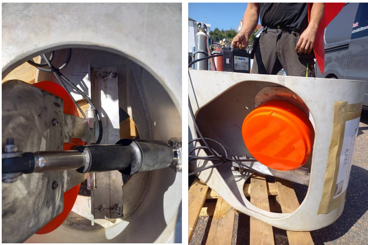
Figure 5. Detail of the hydraulic piston that will provide with tilt for the transducer (left) and transducer inside the blister (right).
