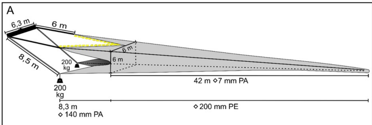
Figure 6. The survey trawl with a 7 mm meshed inner net made of polyamide (PA) 140 mm meshed PA net in the mouth, and 200 mm meshed outer support net in polyethylene (PE). See also Figure 2. In Krafft et al.2018.
