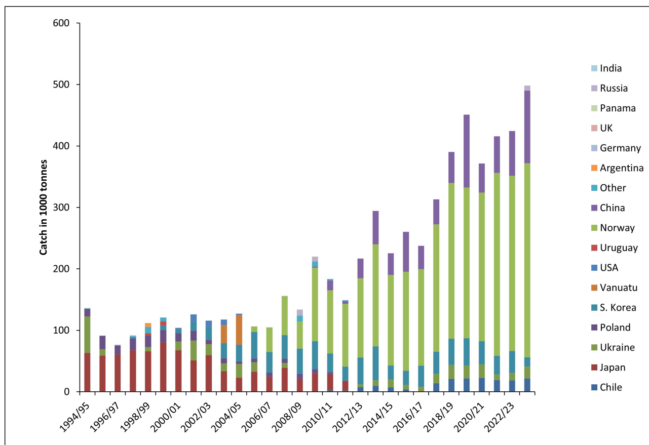
Figure 3. Annual total catch per krill fishing participating flag state in CCAMLR subareas 48.1-4 from the 1994/95 season to the 2023/24 season (data source: ccamlr.org).
