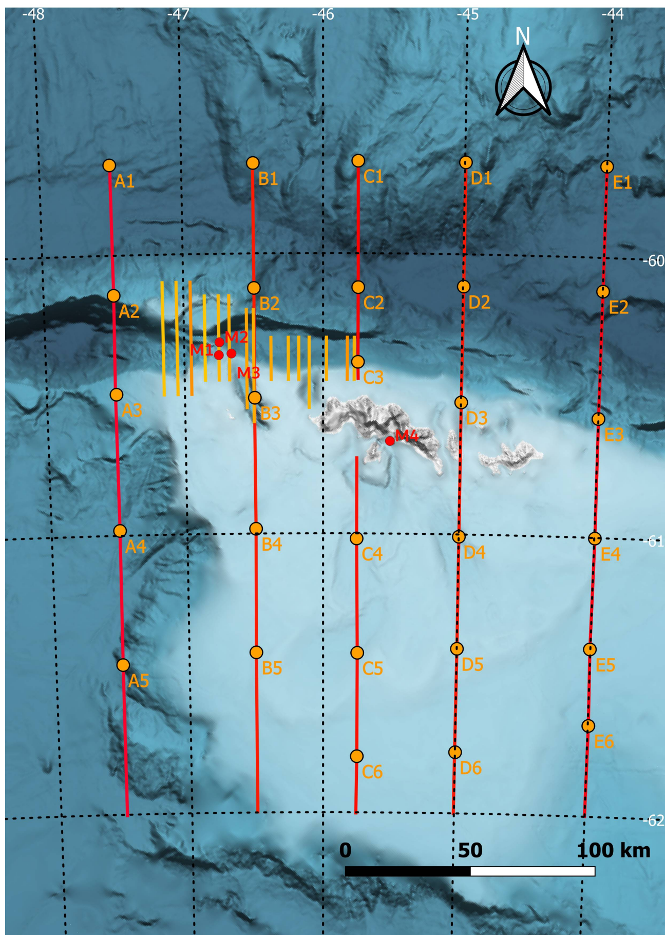
Figure 5. Summary of the 2025 krill monitoring survey lines (A-E) and the 28 trawl stations covered (A1 to E6) and the small Shelf
