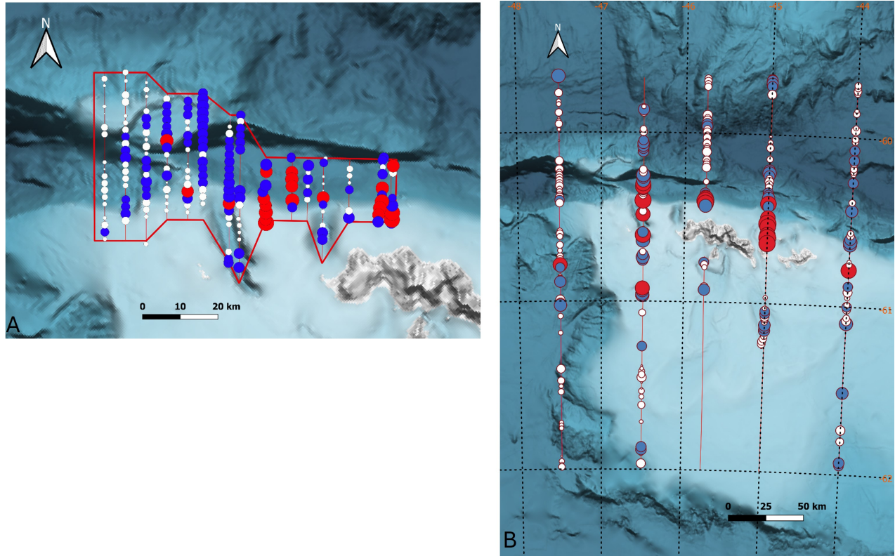
Figure 8. Distribution of Nautical Area Scattering Coefficients (NASC; m 2 /nmi 2 ) allocated to E. superba from the 120 kHz recordings at the Shelf edge stratum (A) and overall stratum (B). Log distance is 1 nautical mile. NASC White: 0-100, Blue: 100-1000 and Red 1000-10000).
