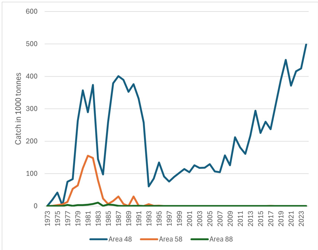
Figure 1. Annual total reported catch of Antarctic krill in the Southern Ocean (data source: ccamlr.org).
