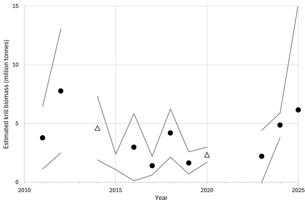
Figure 9. Krill biomass estimates in subarea 48.2 "Overall stratum" 2011-2025. Filled circles are based on 120 kHz acoustic data and open triangles are based on 38 kHz acoustic data. Lines indicate 95% confidence intervals.
