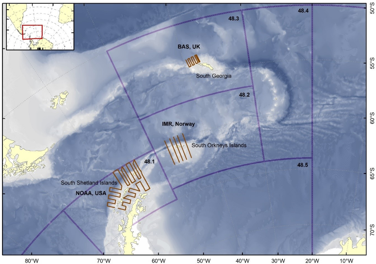
Figure 4. CCAMLR Statistical Reporting Areas 48.1–48.3, with transect lines regularly surveyed for Antarctic krill abundance and demographic composition.
