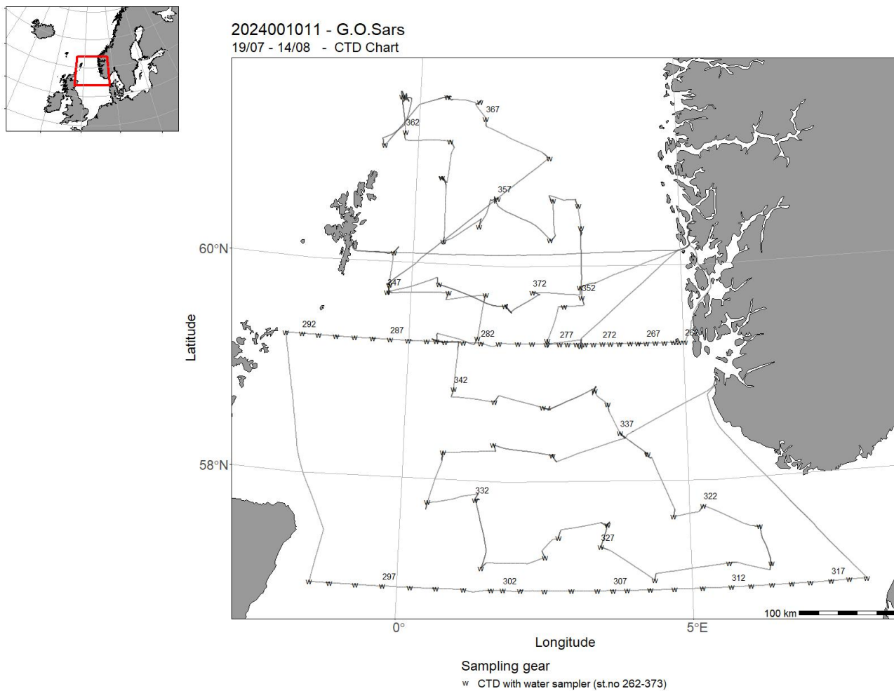
Fig 3.16 CTD chart for 2024001011
