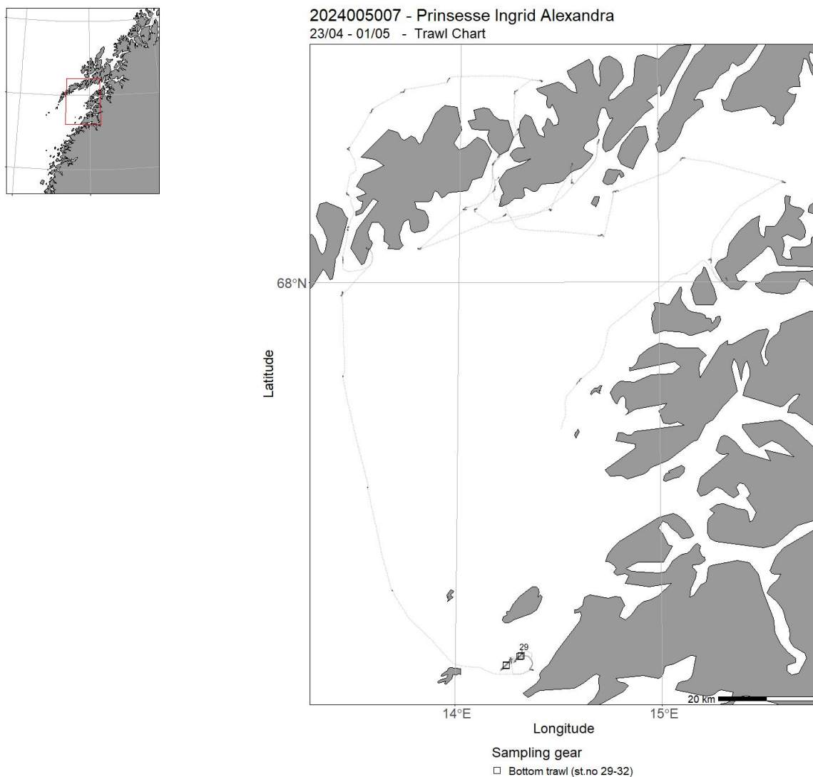
Fig 14.6 Trawl chart for 2024005007
