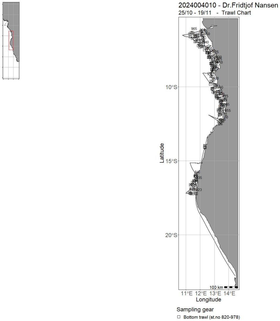
Fig 11.19 Trawl chart for 2024004010
