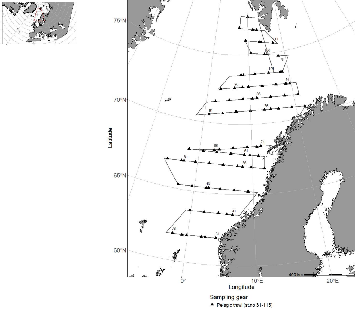
Fig 18.6 Trawl chart for 2024203003
