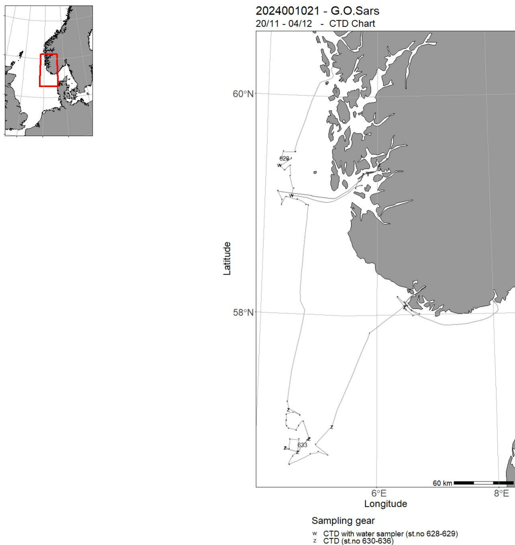
Fig 3.29 CTD chart for 2024001021
