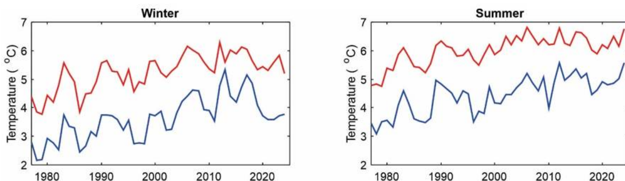
Figure 1.2. Temperature in the AW flowing into the Barents Sea in Fugløya-Bear Island (red) and Vardø-North (blue). Left panels show winter while right panels show summer.
