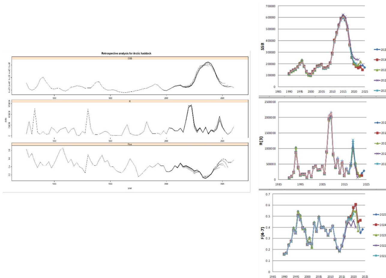
Figure 4.5. Northeast Arctic haddock. Retrospective plots of SSB, fishing mortality and recruitment for assessment years 1950–2024 (left - XSA without P shrinkage, F shrinkage = 0.5) and right - for assessment years 1990–2025 from the TSVPA model.
