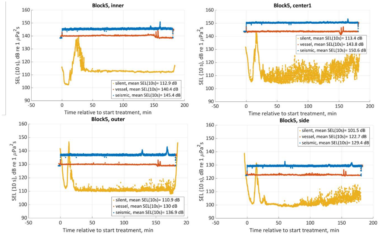
Figure 15 Block 5. Sound exposure levels (SEL) integrated over 10 seconds estimated for every 10 seconds (with 9 seconds overlap) for the duration of each treatment. The levels are a little different from Block 1, probably due to changes in the airgun position.
