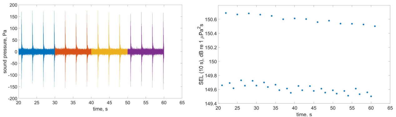
Figure 13. Zoom in on about 40 seconds of sound recording from the centre position. The different colours (left) marks 10 seconds intervals to illustrate that the pulse interval of 3 seconds results in 3 or 4 single seismic pulses pr 10 seconds. The SEL integrated over 10 seconds is affected by the the number of pulses resulting in about 1 dB difference if 3 or 4 pulses is included (right)
