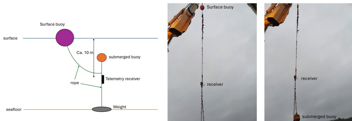
Figure 2 . Illustration (left) of the set up of the telemetry receivers and pictures (right) showing the system when retrieved from the water.
