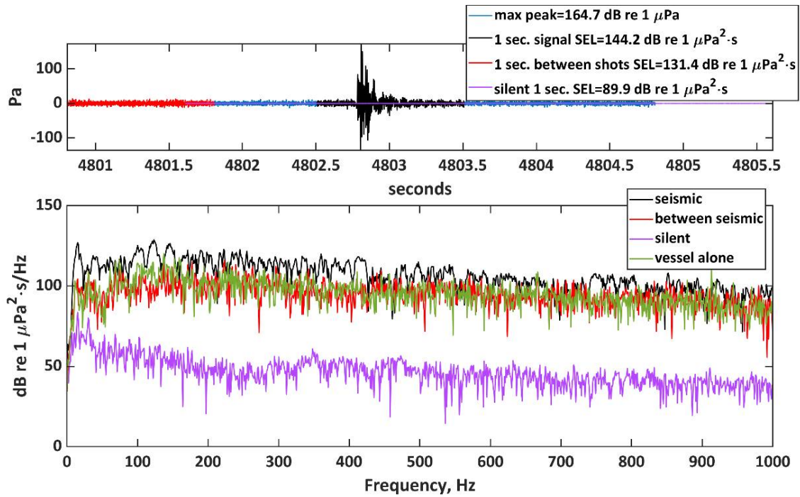
Figure 12. Example of a single seismic signal measured with the Iclisten hydrophone in the centre of the bay. Zero to peak, SEL for the single shot, and SEL for a 1 second duration period before the shot is compared to the silent treatment (see figure legend). In the bottom panel the frequency content of the seismic signal (black1) relative to the period before (red), vessel noise alone (green), and silent with no vessel (purple) is shown. Most of the energy from the seismic is below 450 Hz with the highest levels between 100 – 150 Hz. The signal from the vessel dominates between the seismic signals. The signal from the vessel and vessel + seismic has much higher level than the silent for all measured frequencies, (up to over 20000 Hz). The broadband noise above 500 Hz is probably dominated by the vessel noise since the vessel noise alone shows a similar level.
