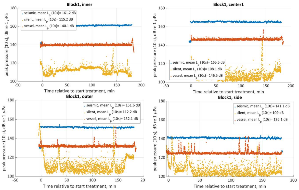
Figure 17. Block 1: Absolute zero to peak sound pressure level estimated as the maximum of the absolute value of the wave form forevery 10 s with 9 s overlap. This is shown for the inner, centre, outer and side position in the bay, for each treatment in Block 1.
