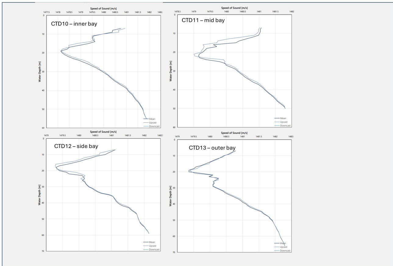
Figure 10. Sound speed profiles for all hydrophone positions from 04.05.2025. Locations are shown in Figure 8 ..
