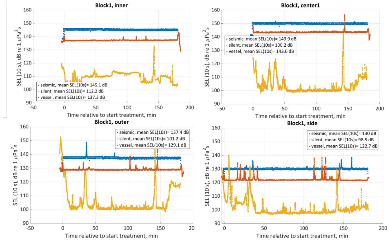
Figure 14. Block 1: Sound exposure levels (SEL) integrated over 10 seconds estimated for every 10 seconds (with 9 seconds overlap) for the duration of each treatment.
