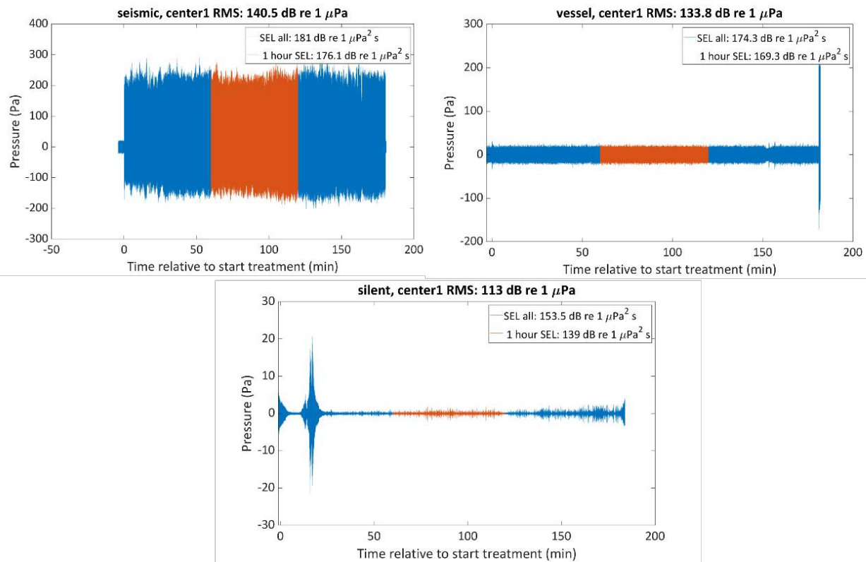
Figure 16. Example of the waveform of the recording for 3 hours of data for the three exposure types. The SEL for 1 hour (in the centre of the treatment marked in orange) is 176.1 dB re 1 \mu Pa 2 s and 181 dB re 1 \mu Pa 2 s for 3 hours of seismic exposure measured in the centre of the bay for Block 5.
