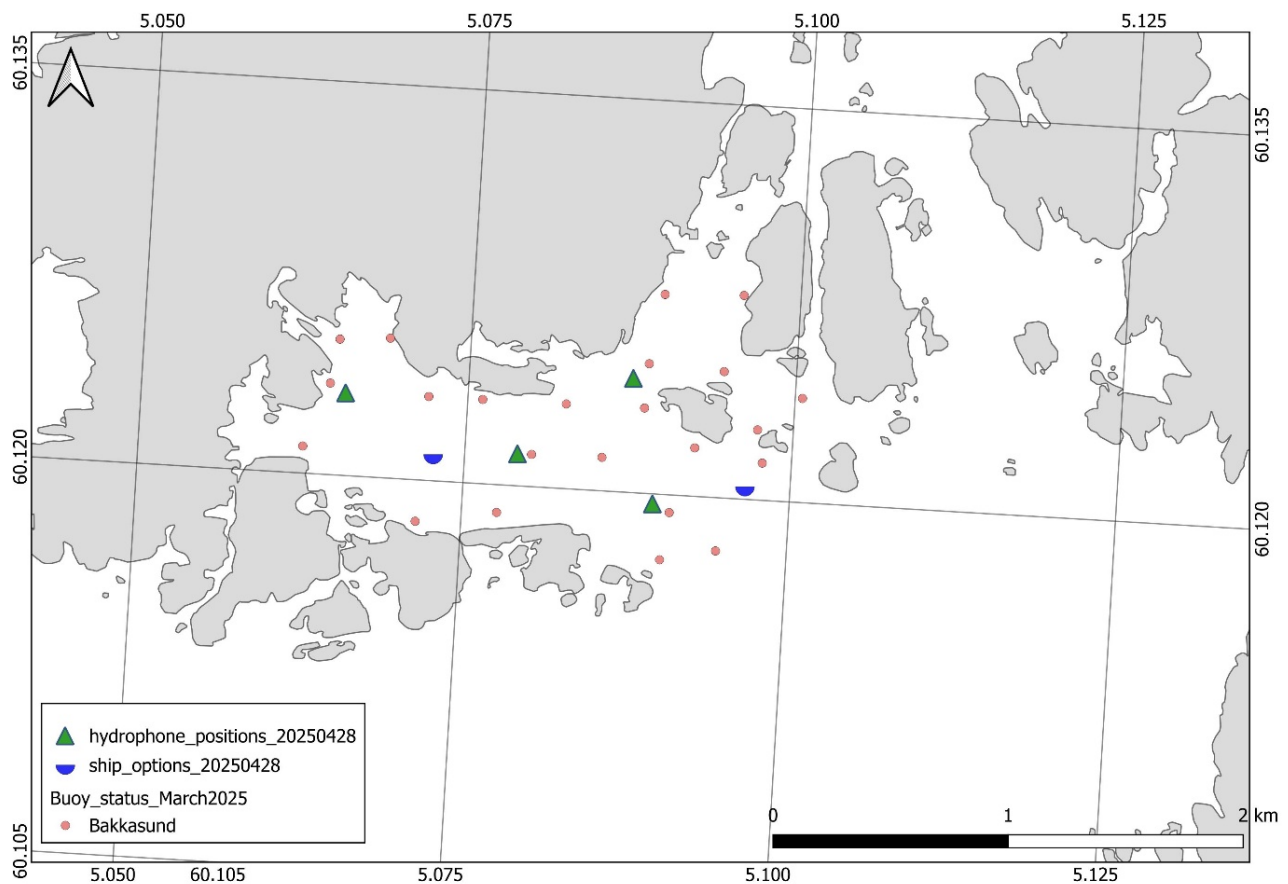
Figure 7. Map of the bay showing the positions of the telemetry receivers (red circles) and placement of hydrophones (green triangles). The hydrophone positions are located approximately 50 m from the telemetry receivers. Two alternative locations of the vessel to be positioned are shown as blue half circles. The preferred option is the one furthest into the bay which was used in this experiment.
