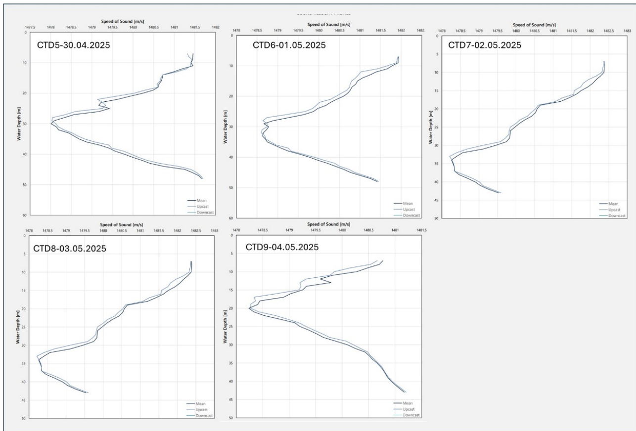
Figure 11. Sound velocity profiles from vessel position at the dates 30.04-2025 – 04.05.2025. Locations are shown in Figure 8 .
