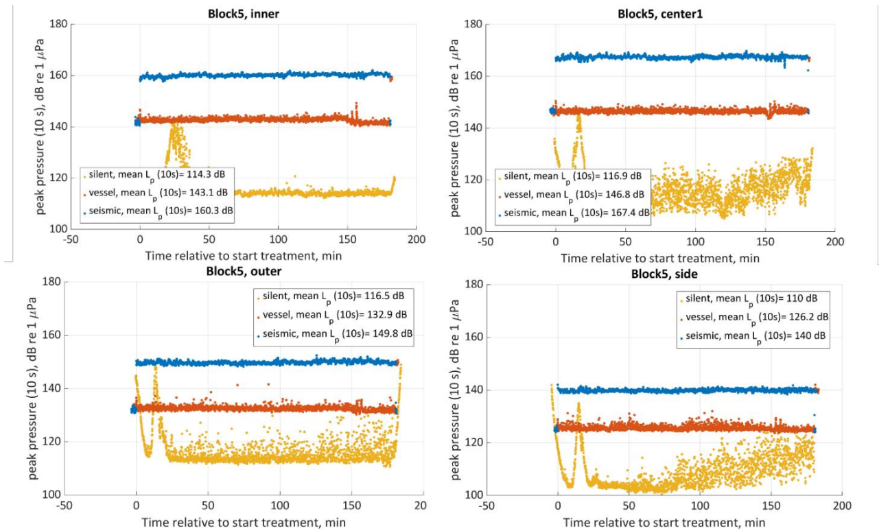
Figure 18. Block 5: Absolute zero to peak sound pressure level estimated as the maximum of the absolute value of the wave form for every 10 s with 9 s overlap. This is shown for the inner, centre, outer and side position in the bay, for each treatment in Block 5. The noise in the silent period can be local boat traffic in the bay.
