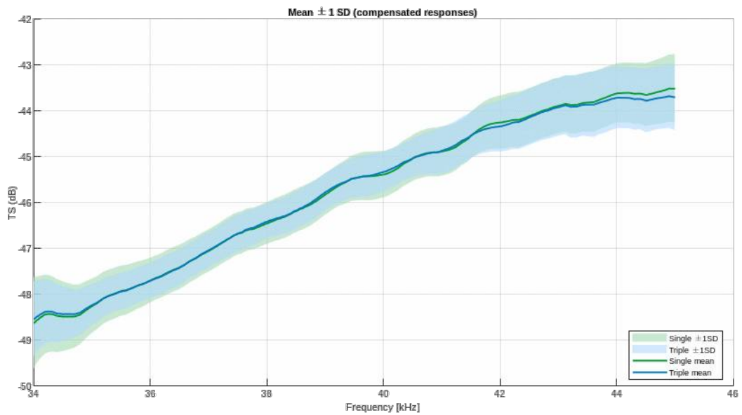
Figure 14 . Estimated TS as a function of frequency for WC25-WO14583 with single and triple suspension using 38 kHz FM.
