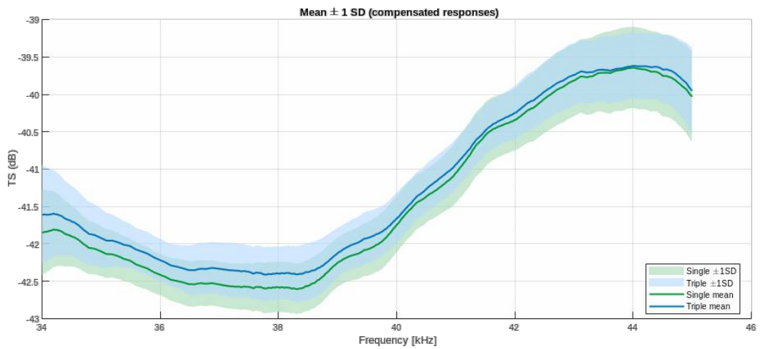
Figure 8 . Estimated TS as a function of frequency for WC38.1-IMR023 with single and triple suspension using 38 kHz FM.
