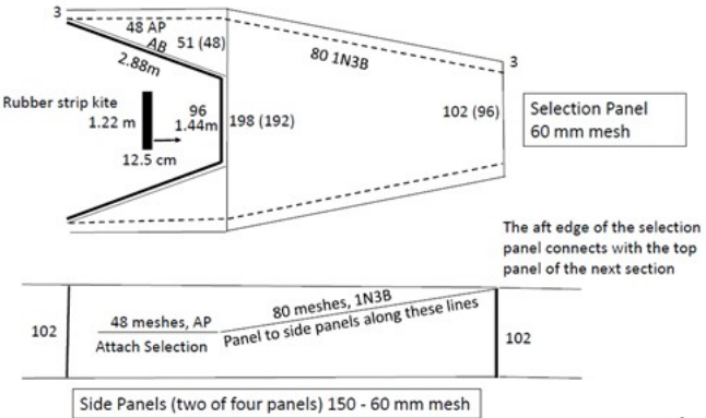
a. Selection Panel Section for Harstad Trawl (last section before codend)
