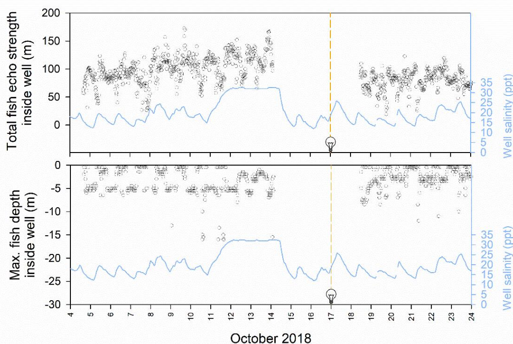
Figure 8. From the freshwater lens pool of a single well cage, measurements of total fish echo signal strength (top plot) and the depth band with the maximum fish echo signal strength (bottom plot, black open circles) plotted over time from 4–24 October 2018. Mean hourly salinity at 1 m within the freshwater lens well pool is also shown (blue lines). Lights within the well pool were installed from 17 October. Tick marks on the x axis are position at 0000 h.
