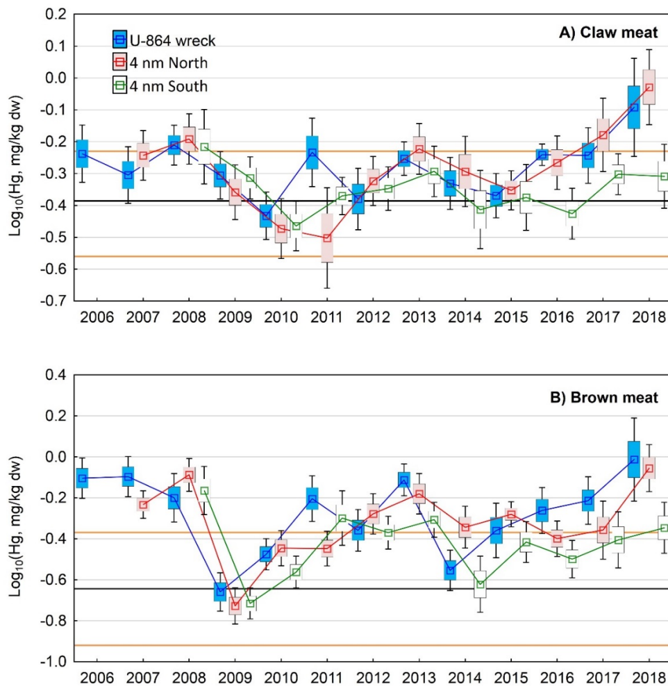
Figure 5. Concentrations (mg/kg dry weight, dw) of Hg over time from 2006-2018 analysed in A) claw meat and B) brown meat of boiled crabs captured at the site of U-864, 4 nautical miles (nm) south and 4 nm north of the wreck. Concentrations are given as \log_{10} transformed values, and mean, standard errors and 95% confidence intervals are given. The horizontal lines represent reference sites on the west coast of Norway south of 62°N. The black horizontal line represents the mean Hg concentration of all 110 crab samples analysed in 2011 on the coast of west Norway south of 62°N (Julshamn m.fl. 2012). The orange lines represent the highest and the lowest mean values among all 11 stations included in the study.
