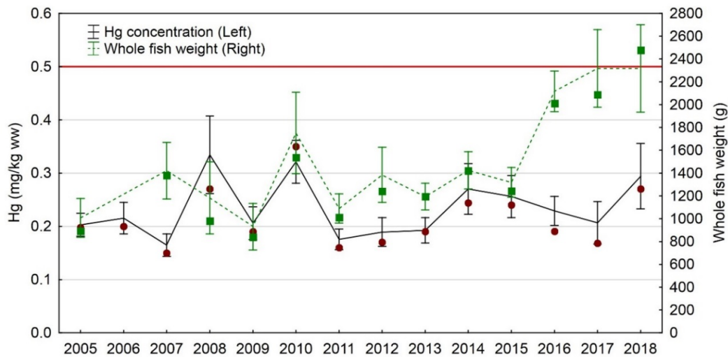
Figure 2. Concentration of mercury (mg/kg ww, left) in fillet and fish weight (g, right) of tusk ( Brosme brosme ) caught near the wreck of U-864 every year from 2005-2018. For each year, mean \pm 95% confidence intervals are given, and median values are shown as separate points. The red line marks the maximum level for Hg in fish for human consumption (EU and Norway).
