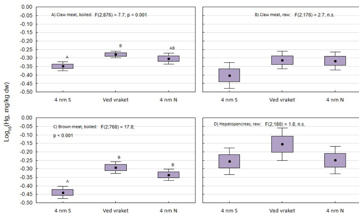
Figure 5. Total mercury concentration on dry weight (Hg, mg/kg dw) in crab ( Cancer pagurus ) caught at the wreck of U-864 (U-864), four nautical miles north of the wreck (4 nm N) and four nautical miles south of the wreck (4 nm S) during 2006-2020. Results are given for A) claw meat of boiled crab, B) claw meat of raw crab, C) brown meat of boiled crab and D) hepatopancreas of raw crab. Boxplots show mean, standard error and 96% confidence intervals of \text{log}_{10} transformed values. Results of one-way ANOVA is given with significance level of 95%. Different letters above the boxes indicate significant differences between groups (Tukey HSD).
