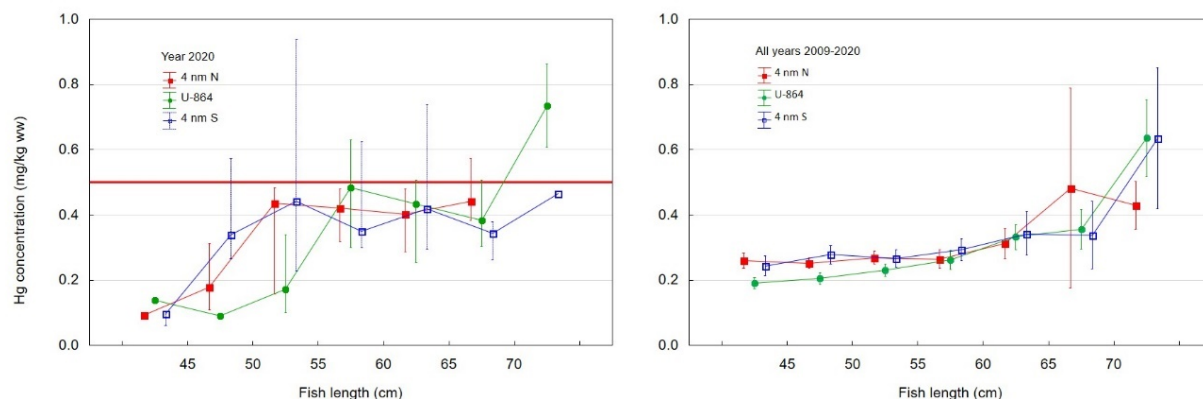
Figure 3. Concentration of mercury (mg/kg ww; mean and confidence interval) in fillet of tusk ( Brosme brosme ) at different length intervals (<45, 45-50, 50-55, 55-60, 60-65, 65-70 and >70 cm), caught at three different sites; at the wreck of U-864, four nautical miles south (4 nm S) and four nautical miles north (4 nm N) of U-864. Left: Year 2020 only, median, minimum and maximum values shown. Right: All years 2009-2020, means \pm 95% confidence intervals are given.
