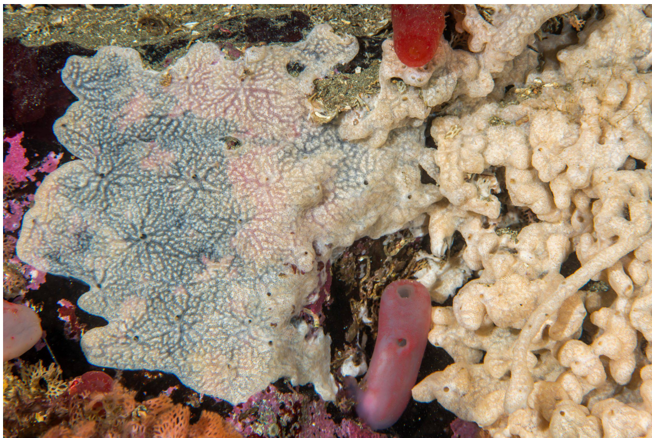
Figure 9. Didemnum vexillum . Photo: Erling Svensen.
