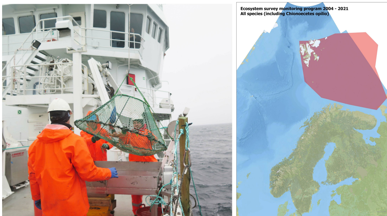
Figure 3. (left) Pot-fishing of snow crab. Photo: Ann-Merete Hjelseth. (right) Monitoring area of snow crab through the Ecosystem Survey Monitoring Program 2004-2021. Red area indicates area which is investigated.
