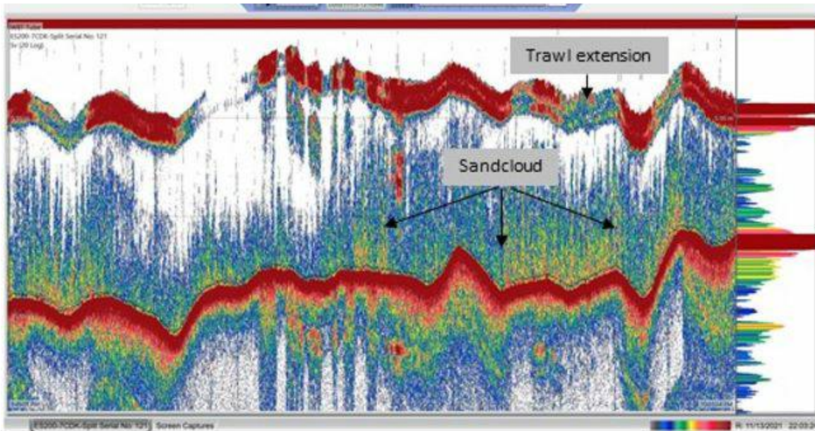
Figure 9 . Examples of EK80 data from echosounder mounted under the FOCUS-2 vehicle. The FOCUS was 2 – 30 m above the trawl and the sand cloud can be observed below and inside the trawl. The first image is from approaching the trawl and measuring the first part of the trawl. Range is 70 m. The image in the middle is showing cross sections of the trawl middle part and sand cloud under and inside the trawl. The range is 40 m. In the image on the bottom FOCUS is 2 – 5 m above the trawl extension which is about 10 meters above the seafloor. The sand cloud can be seen below the trawl extension. Range is 20m.
