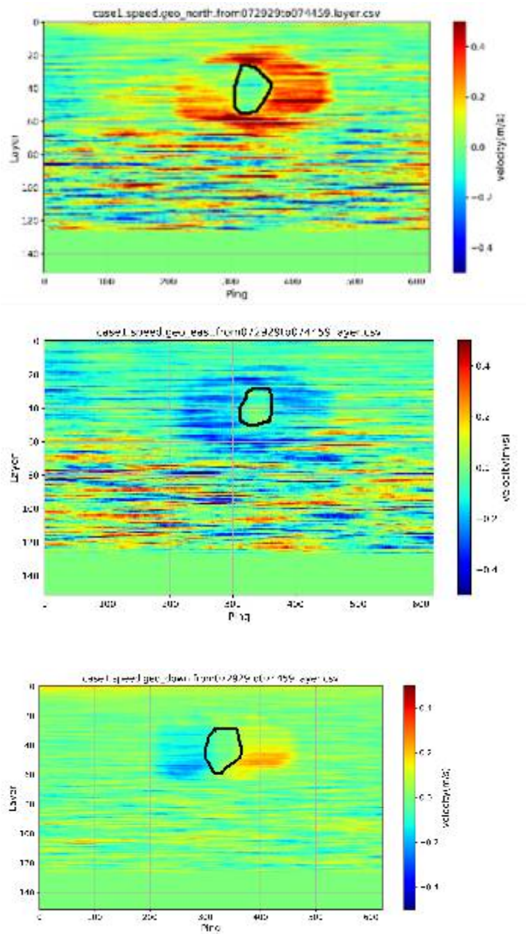
Fig. 15. Data selection over the valid pings in north-south (upper panel), east-west (middle panel) and up-down (lower panel) directions.
