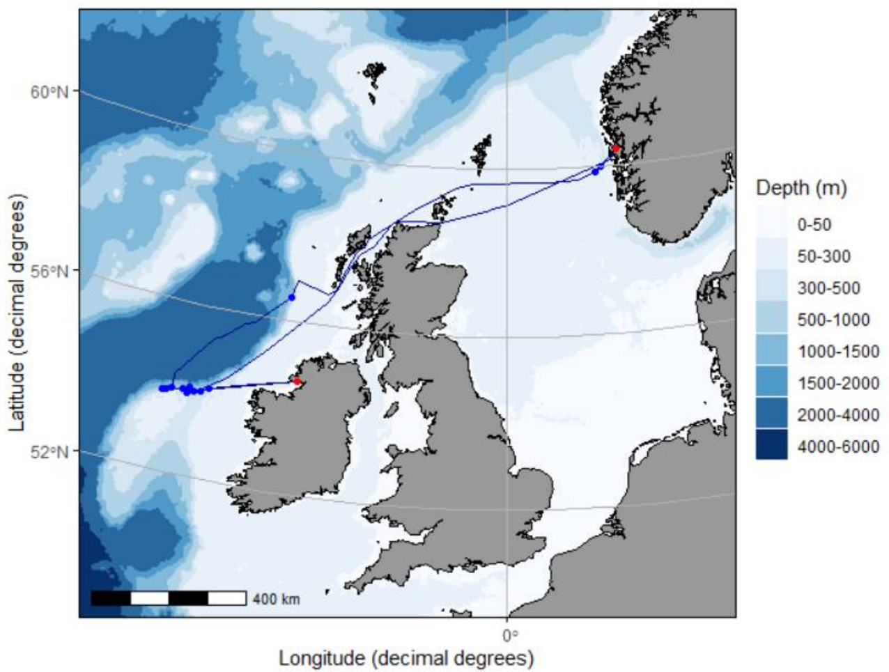
Fig. 13.22 - Cruise track for cruisenum 2021825, Vikingbank. Trawl hauls are indicated with blue points and red points indicate harbours visited (Bergen, Norway, and Killybegs, Eire).
