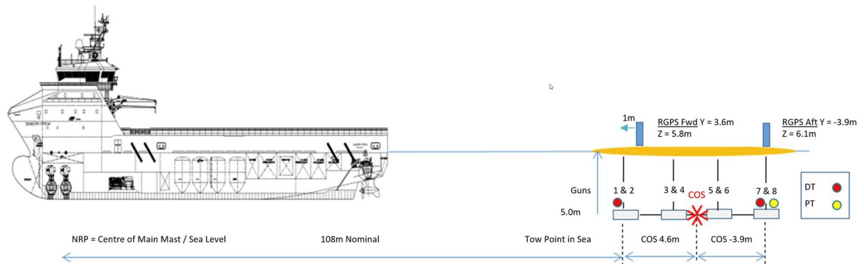
Figure 15. The two drawings show the dimension of the seismic air gun and its positioning in the water and in relation to the seismic vessel.
