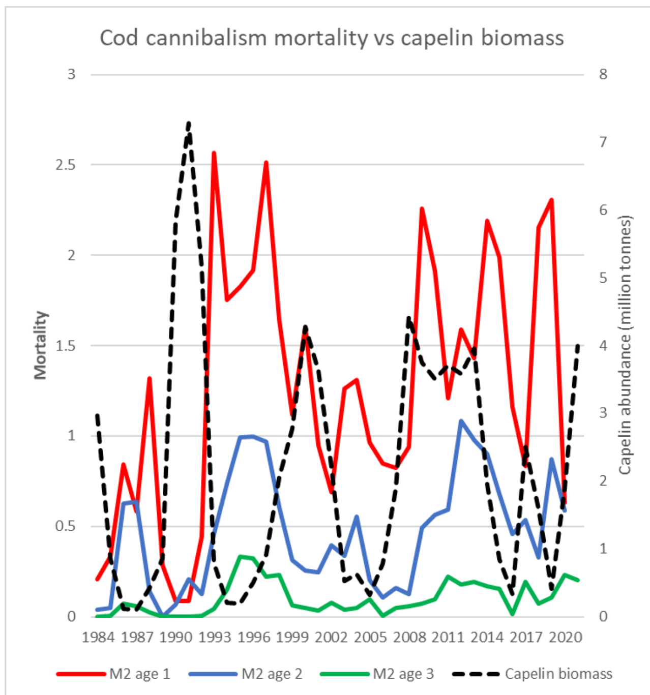
Figure 3.3. NEA cod cannibalism mortality vs. capelin abundance.
