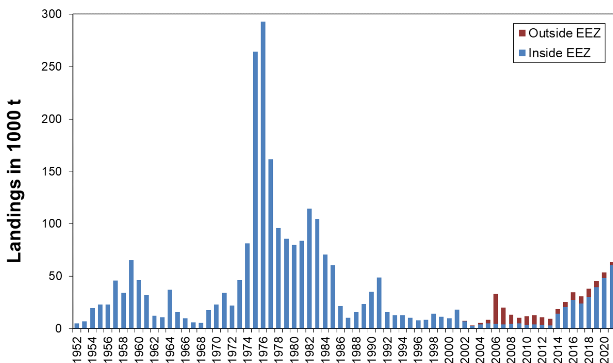
Figure 6.1. S. mentella in subareas 1 and 2. Total international landings 1952–2020 (thousand tonnes).
