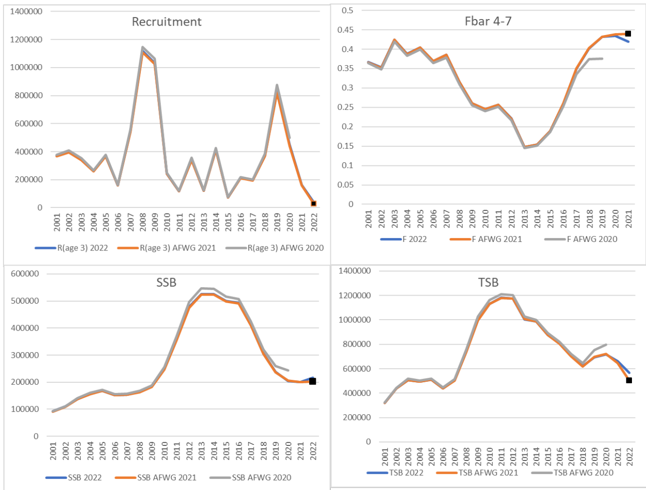
Figure 4.4. Results of assessment of NEA haddock. F_{bar}(4-7) , TSB, recruits and SSB from AFWG 2020 (grey), AFWG 2021 (orange) and this year's (2022) assessment (blue) from 2001 and onwards. The last black squares on the lines for AFWG 2021 (orange) are forecasts for 2022 made last year. .
