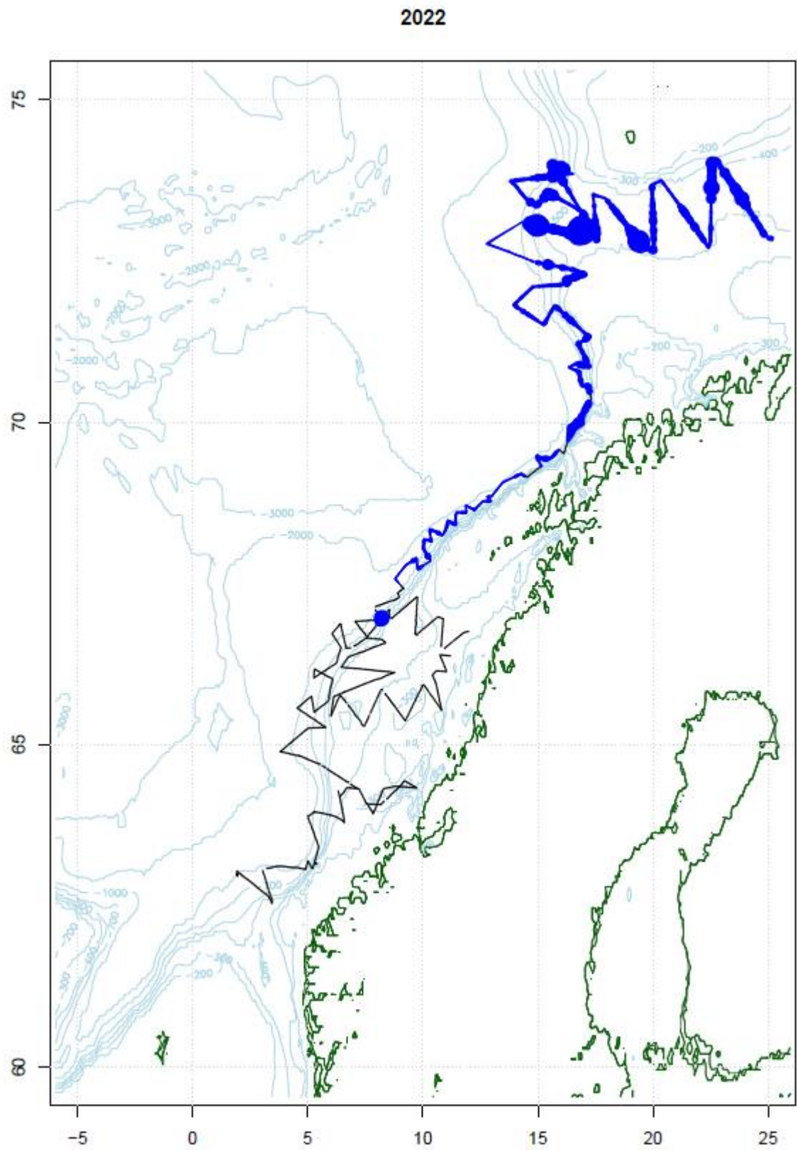
Figure 6.17. S. mentella in subareas 1 and 2. Horizontal distribution of S. mentella hydroacoustic backscattering (sA) during the Norwegian slope survey in spring 2022. The circles are proportional to the sA assigned to redfish along the vessel track.
