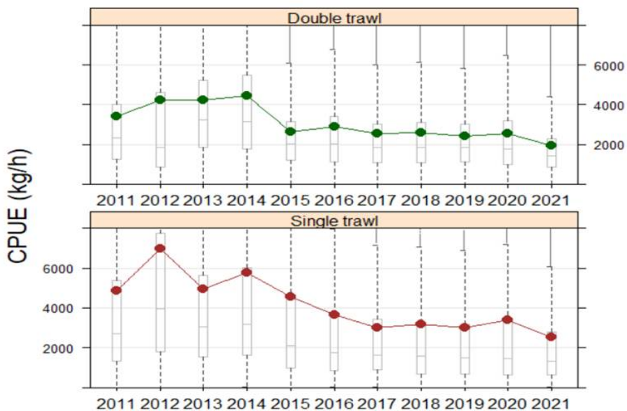
Figure 3. 5. Cod CPUE in Norwegian trawl catches where cod is the main species (double and single trawl). Connected line shows mean, line inside the box shows the median, and the box shows 25 and 75 percentiles.
