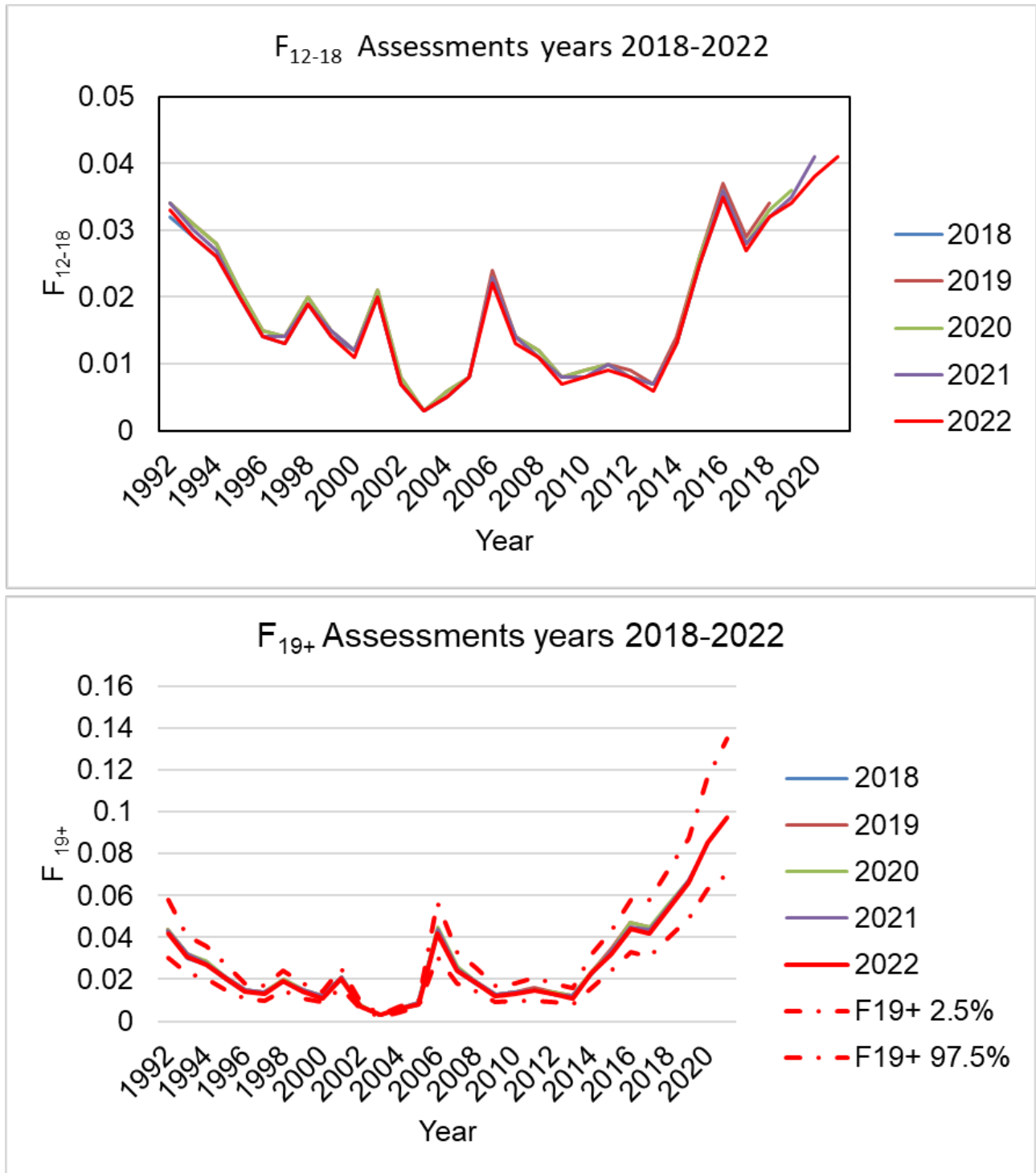
Figure 6.25. The upper panel shows the retrospective patterns of the fishing mortality for the age classes 12-18, estimated by the SCAA model for runs up to years 2018-2022. The lower panel presents fishing mortality for the age-19+ group for the same time period. Broken lines indicate the confidence intervals for the 2022 assessments.
