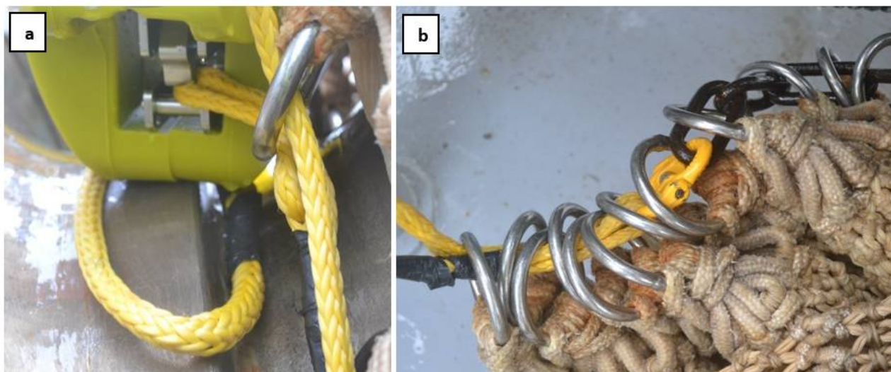
Figure 7.5 – Observations after test C-2 (rig 2); a: the soft eye was only partially released from the reaser jaw; and b: the hammerlock linking the Dynaema twine to the securing chain was jammed in the cod-end skirt rings.
