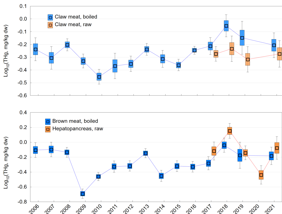
Figur 5. Concentrations (mg/kg dry weight, dw) of total mercury (THg) from 2006-2021 analysed in A) claw meat and B) brown meat of raw (orange) and boiled (blue) crabs captured at the site of U-864 and 4 nautical miles north of the wreck. Concentrations are given as \text{log}_{10} transformed values, and mean, standard errors and 95% confidence intervals are given. From 2018 on, samples were not freeze dried before analysis, and dry matter was determined by drying at 104°C.
