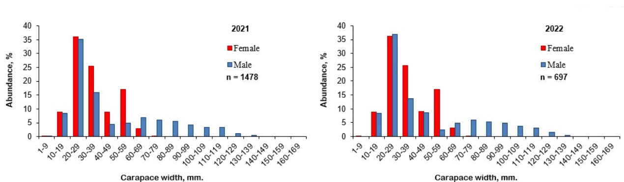
Figure 10.3.2. Size and sex structure of the snow crab in the Barents Sea in August-December 2021- 2022 (by BESS data).
