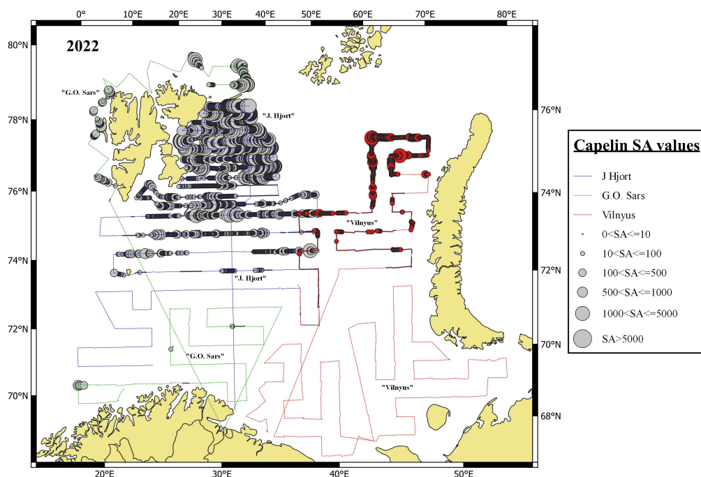
Figure. 7.1.1.1. Geographical distribution of capelin in autumn 2022 based on acoustic recordings. Circle sizes correspond to S_A values ( m^2/nmi^2 ) per nautical mile. The circles and transect marked with red colour are recordings from Vilnyus made later than the other vessels (see text for details).
