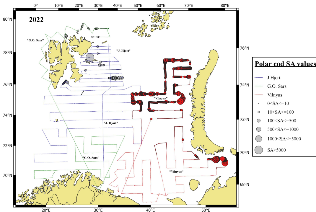
Figure 7.2.1.1 Geographical distribution of polar cod in autumn 2022 based on acoustic data. Circle sizes correspond to s_A values ( m^2/nmi^2 ) per nautical mile. The circles and transect marked with red colour are recordings from Vilnyus made later than the other vessels (see text for details).
