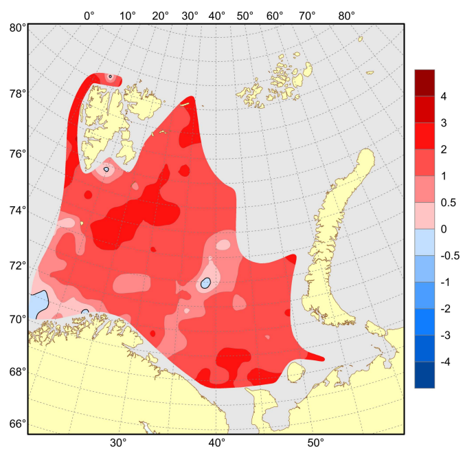
Figure 4.1.1.9. Surface temperature anomalies (°C), August–November 2022.
