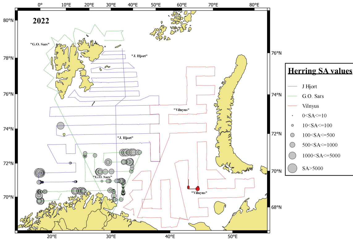
Figure 7.3.1.1 Geographical distribution of herring in autumn 2022 based on acoustic recordings. Circle sizes correspond to s_A values ( m^2/nmi^2 ) per nautical mile. The circles and transect marked with red colour are recordings from Vilnyus made later than the other vessels (see text for details).
