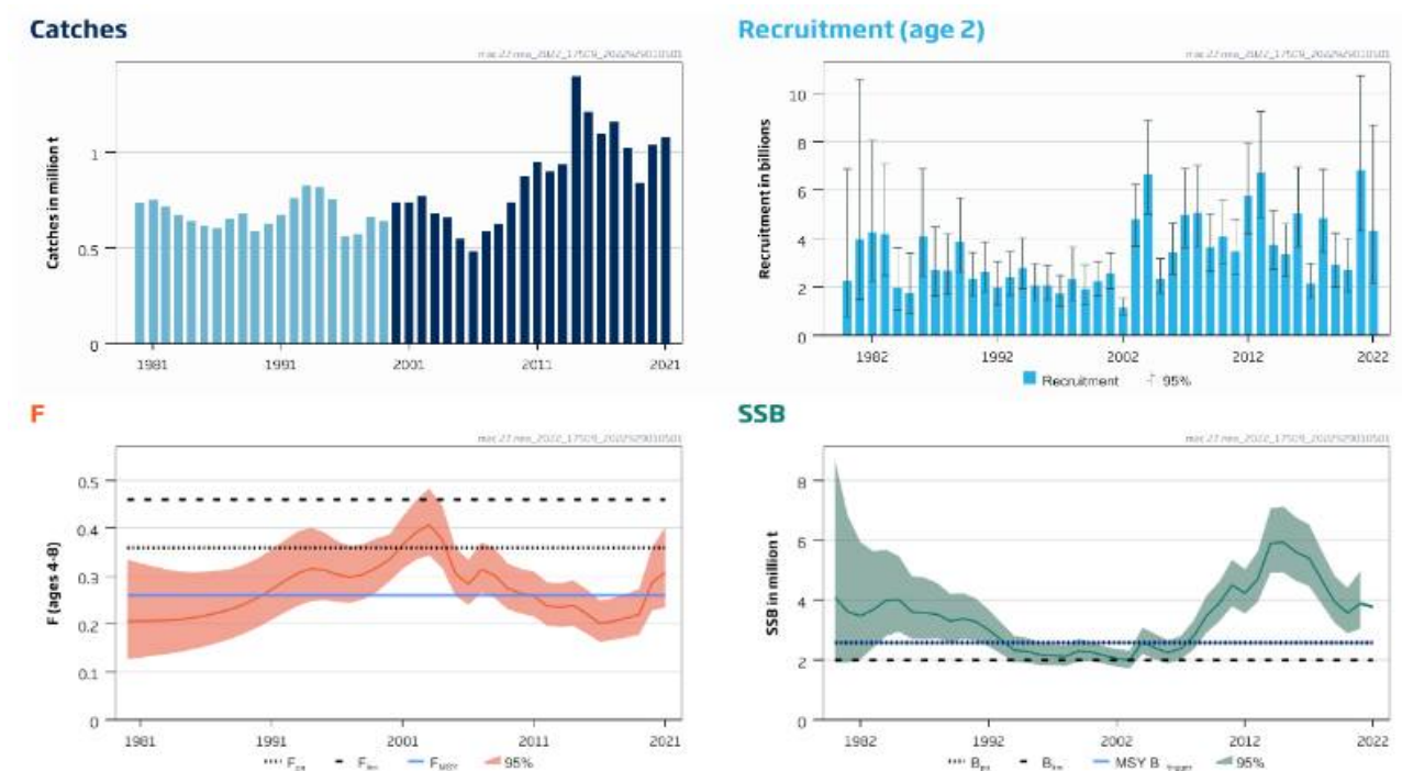
Figure D.1.1 Mackerel in subareas 1–8 and 14, and in Division 9.a. Summary of the stock assessment. Catches prior to 2000 have been down-weighted in the assessment because of the considerable underreporting suspected to have taken place in this period. Abundance estimates of age 0 and 1 from the assessment model poorly reflect year-class strength and therefore recruitment is shown at age 2. Source: ICES (2022c)
