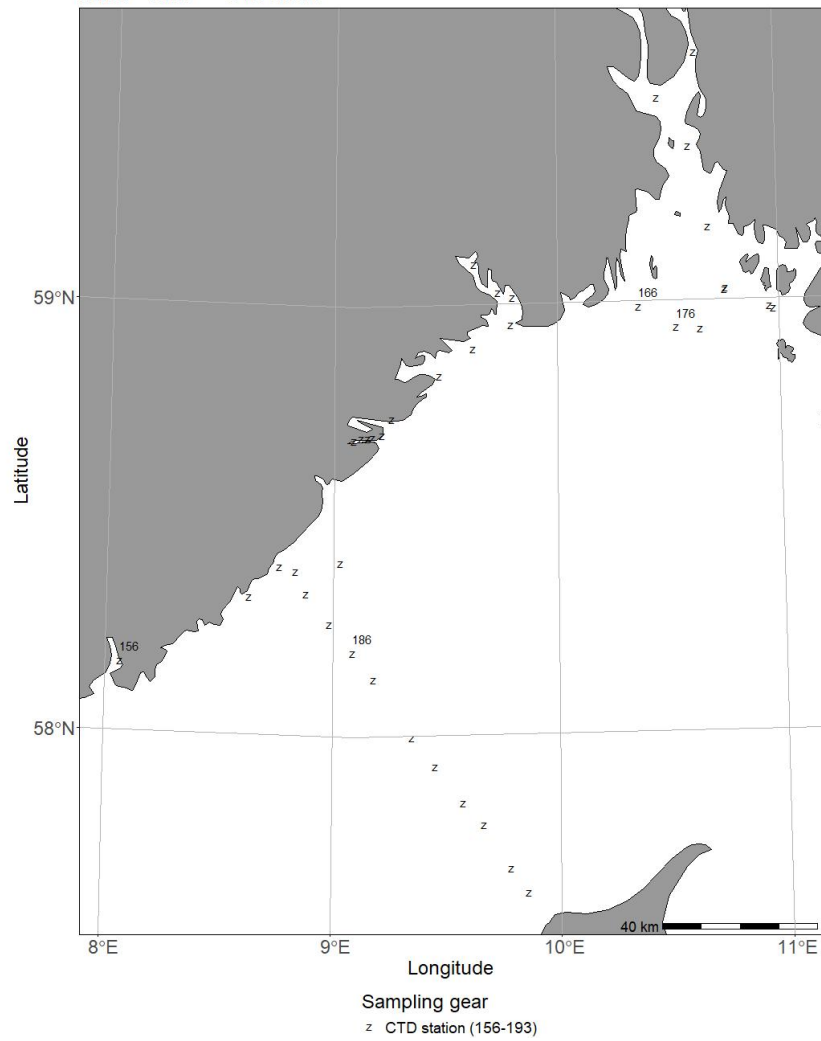
2022309 - G.M.Dannevig 08/06 - 17/06 - CTD Chart
