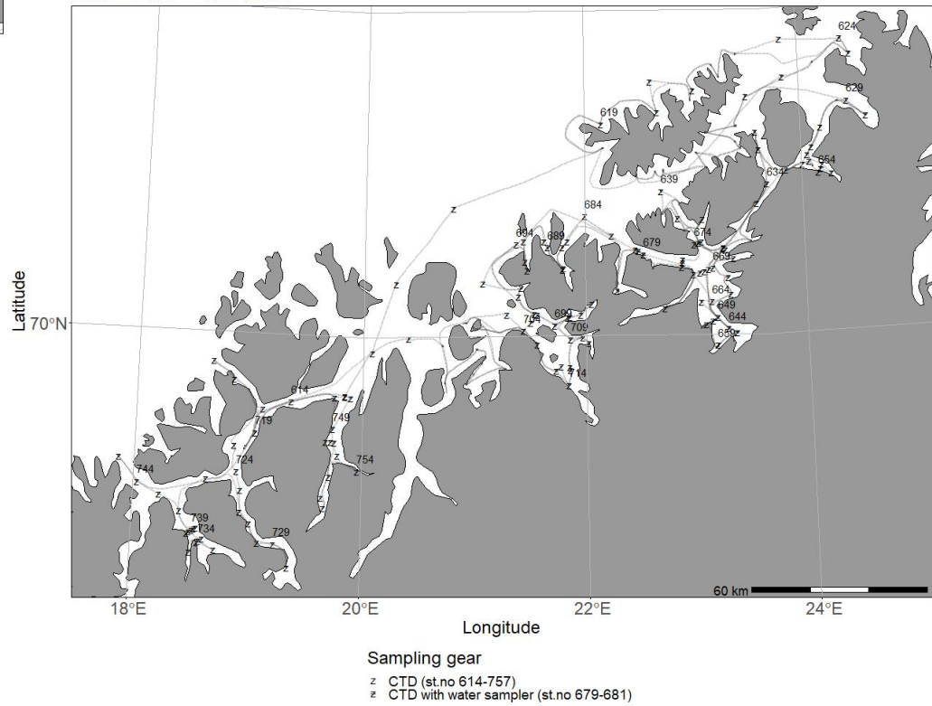
2022615 - Kristine Bonnevie 01/06 - 12/06 - CTD Chart
