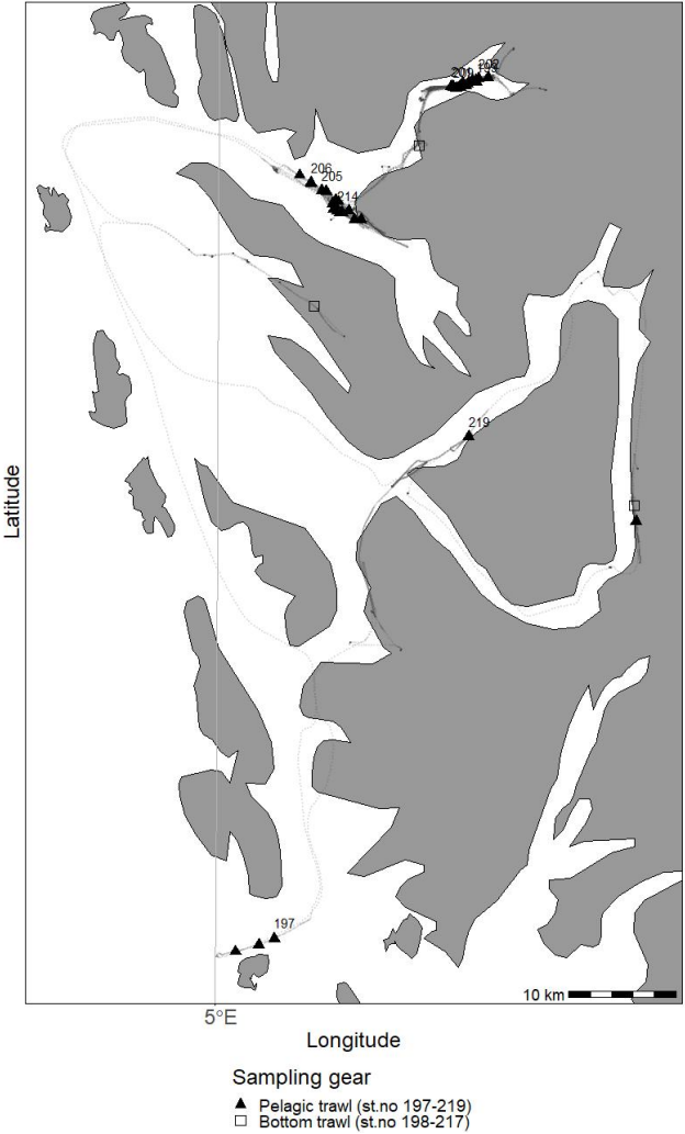
2022614 - Kristine Bonnevie 22/05 - 28/05 - Trawl Chart
