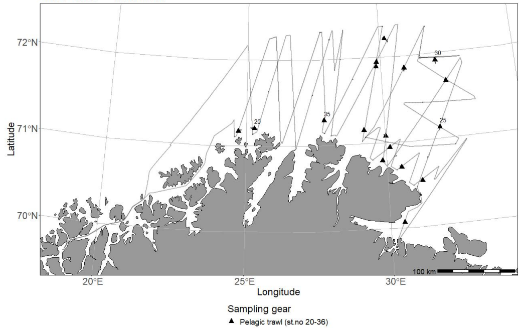
2022802 - Vendla 27/02 - 13/03 - Trawl Chart
