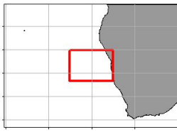
2022405 - Dr.Fridtjof Nansen 11/06 - 12/07 - CTD Chart
