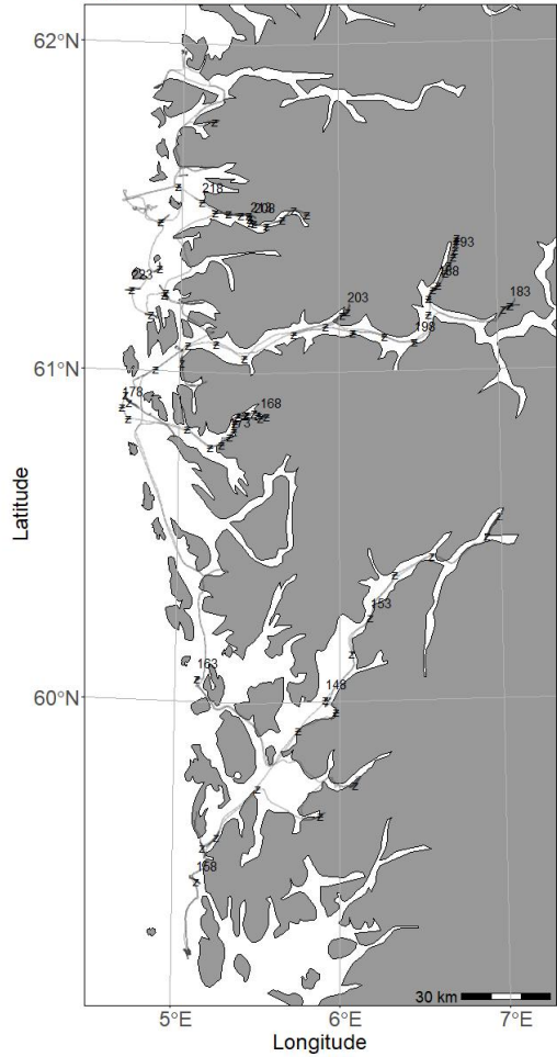
2022603 - Kristine Bonnevie 09/02 - 18/02 - CTD Chart
