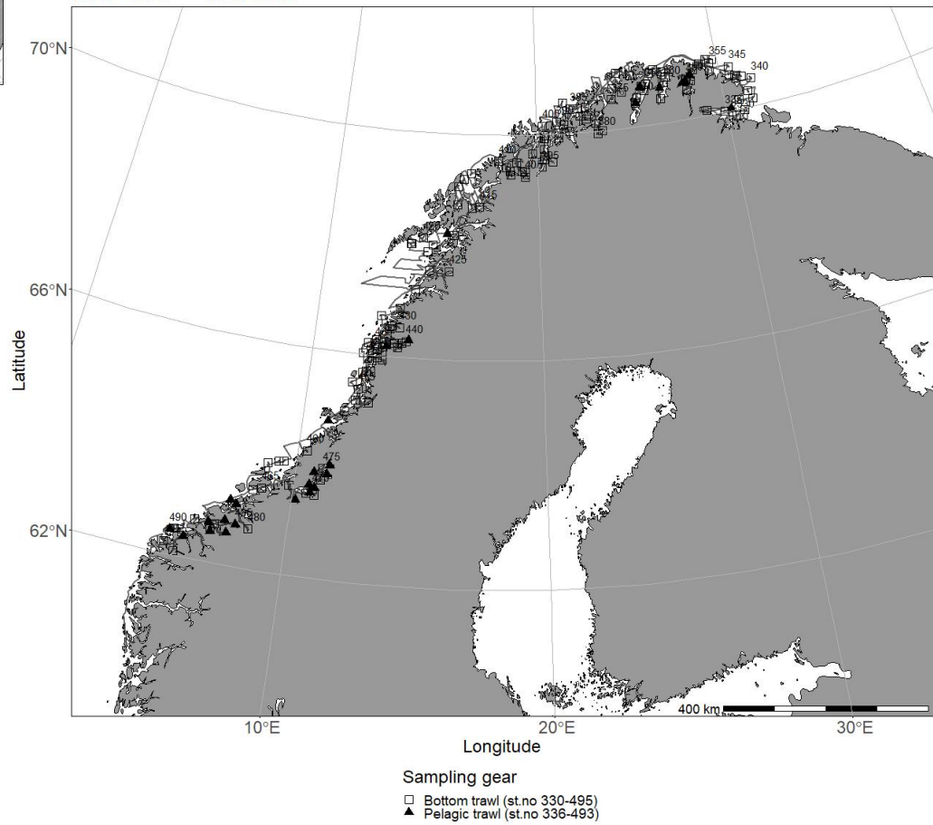
2022626 - Kristine Bonnevie 15/10 - 24/11 - Trawl Chart
