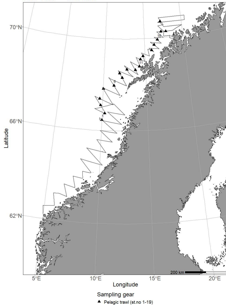
2022821 - Vendla 14/02 - 27/02 - Trawl Chart
