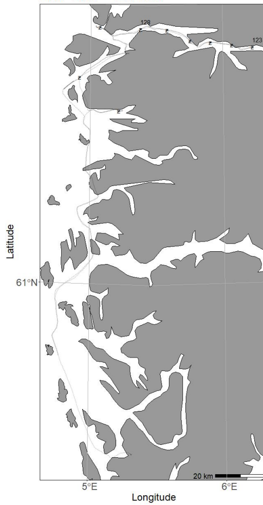
2022102 - G.O.Sars 24/02 - 26/02 - CTD Chart
