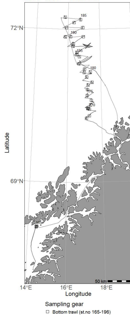
2022609 - Kristine Bonnevie 08/04 - 19/04 - Trawl Chart
