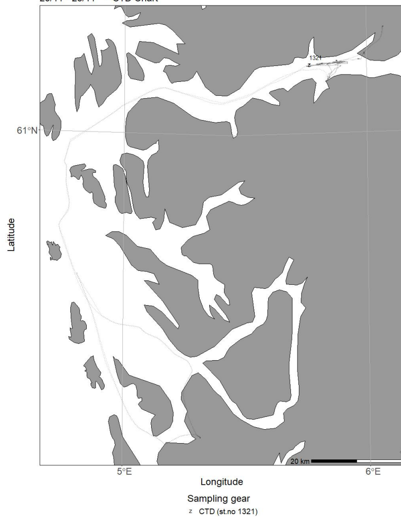
2022622 - Kristine Bonnevie 25/11 - 28/11 - CTD Chart
