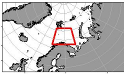
2022204 - Johan Hjort 27/01 - 14/03 - Trawl Chart
