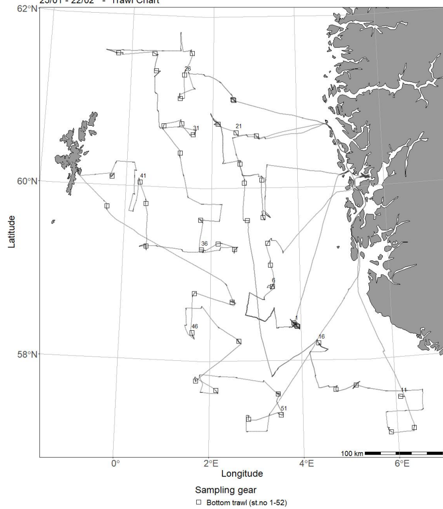
2022101 - G.O.Sars 25/01 - 22/02 - Trawl Chart
