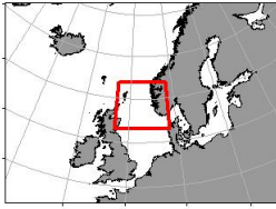
2022619 - Kristine Bonnevie 12/07 - 15/08 - Trawl Chart
