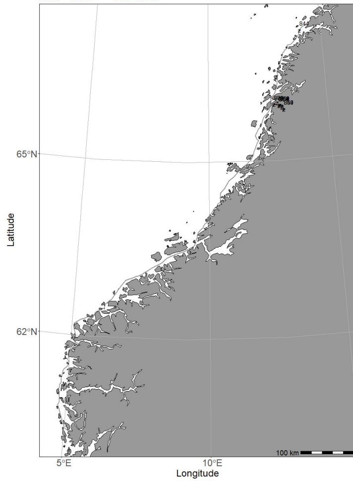
2022618 - Kristine Bonnevie 05/07 - 09/07 - CTD Chart
