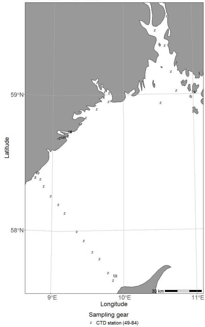
2022303 - G.M.Dannevig 02/03 - 18/03 - CTD Chart
