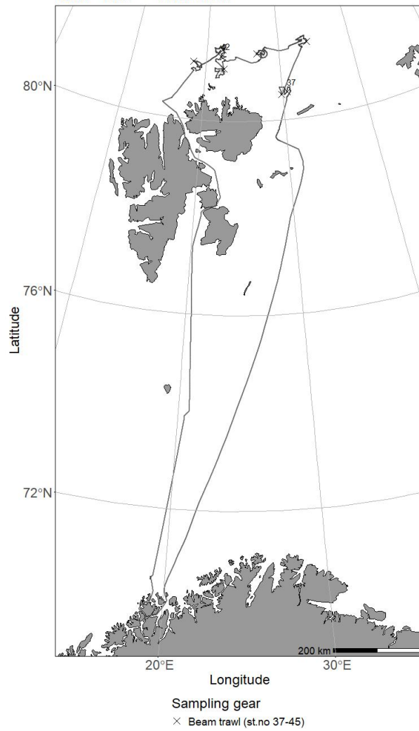
2022708 - Kronprins Haakon 18/06 - 15/07 - Trawl Chart
