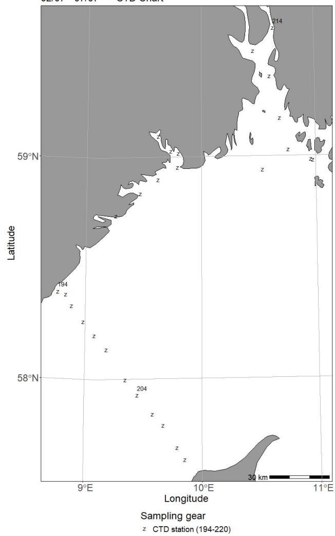
2022310 - G.M.Dannevig 02/07 - 07/07 - CTD Chart
