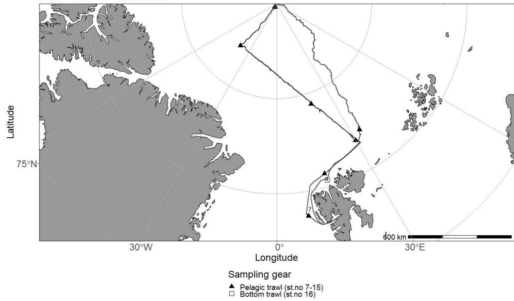
2022710 - Kronprins Haakon 20/07 - 23/08 - Trawl Chart
