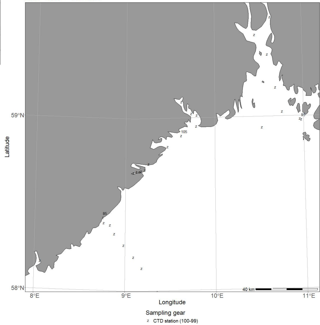
2022305 - G.M.Dannevig 20/04 - 27/04 - CTD Chart
