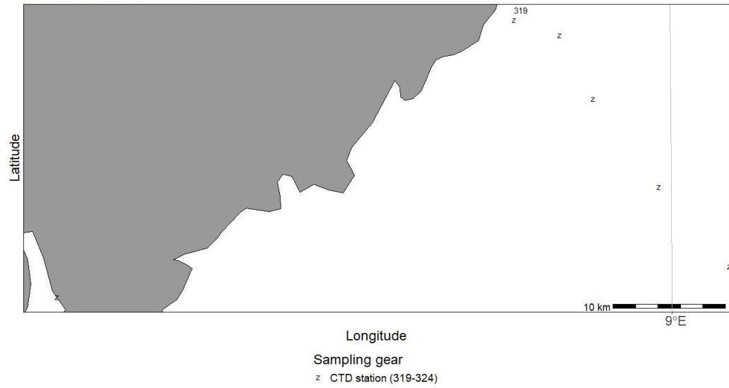
2022316 - G.M.Dannevig 08/10 - 09/10 - CTD Chart
