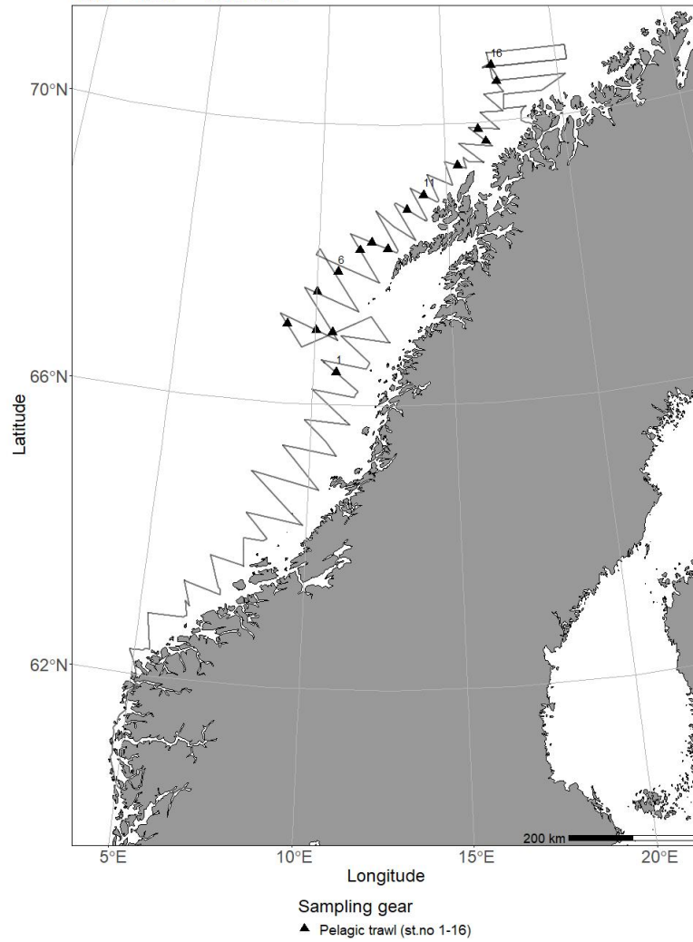
2022822 - Eros 14/02 - 27/02 - Trawl Chart
