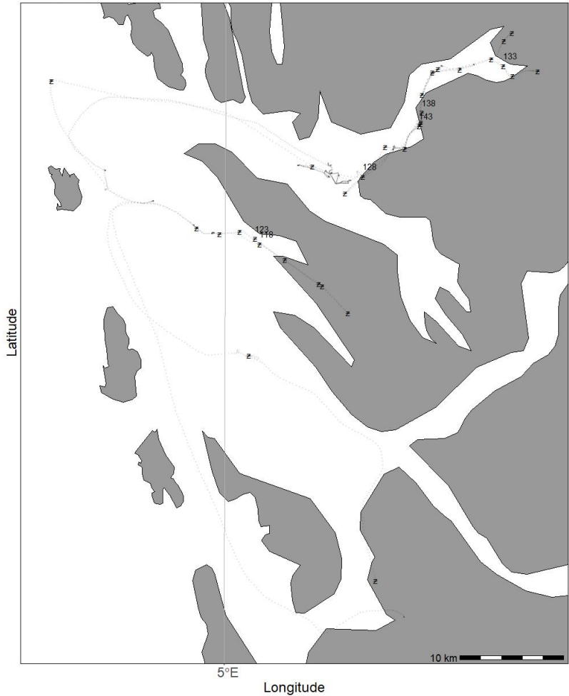
2022602 - Kristine Bonnevie 02/02 - 05/02 - CTD Chart
