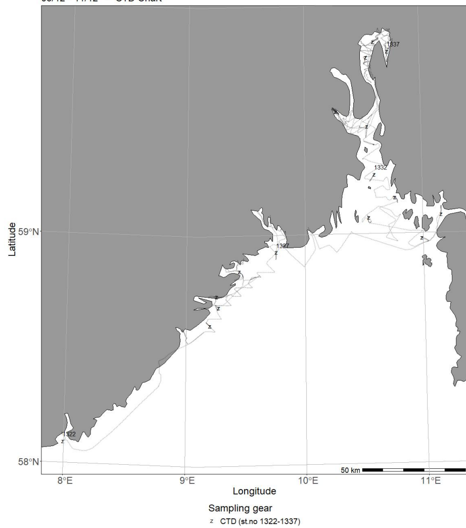
2022628 - Kristine Bonnevie 06/12 - 11/12 - CTD Chart
