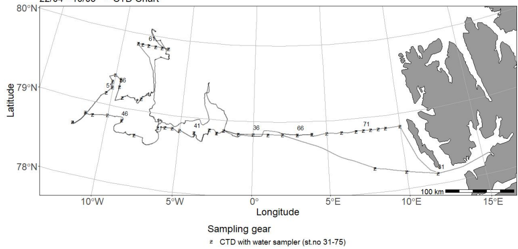
2022704 - Kronprins Haakon 22/04 - 10/05 - CTD Chart
