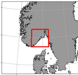
2022315 - G.M.Dannevig 15/09 - 07/10 - CTD Chart
