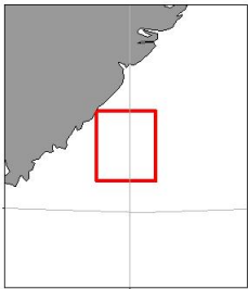
2022314 - G.M.Dannevig 13/09 - 14/09 - CTD Chart
