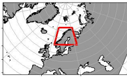
2022626 - Kristine Bonnevie 15/10 - 24/11 - Trawl Chart
