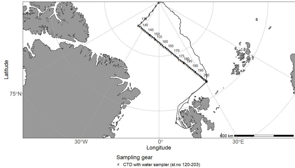
2022710 - Kronprins Haakon 20/07 - 23/08 - CTD Chart
