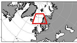
2022105 - G.O.Sars 26/04 - 30/05 - Trawl Chart
