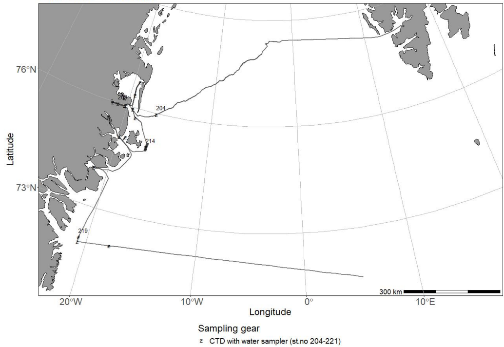
2022715 - Kronprins Haakon 24/08 - 07/09 - CTD Chart
