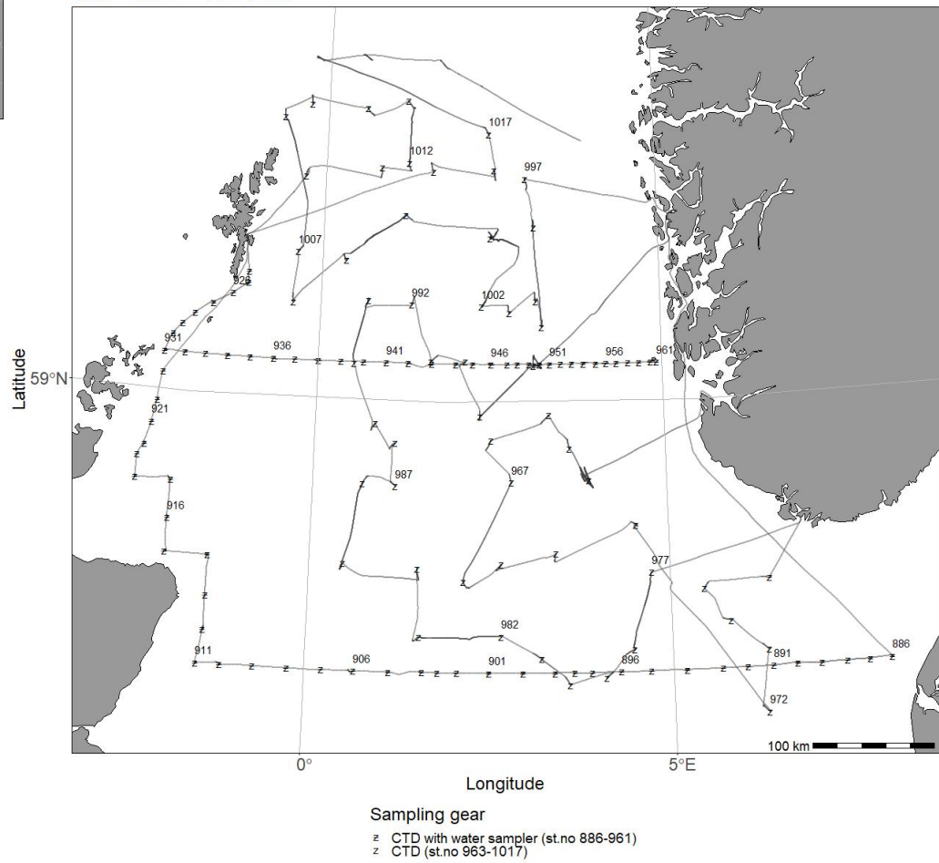
2022619 - Kristine Bonnevie 12/07 - 15/08 - CTD Chart
