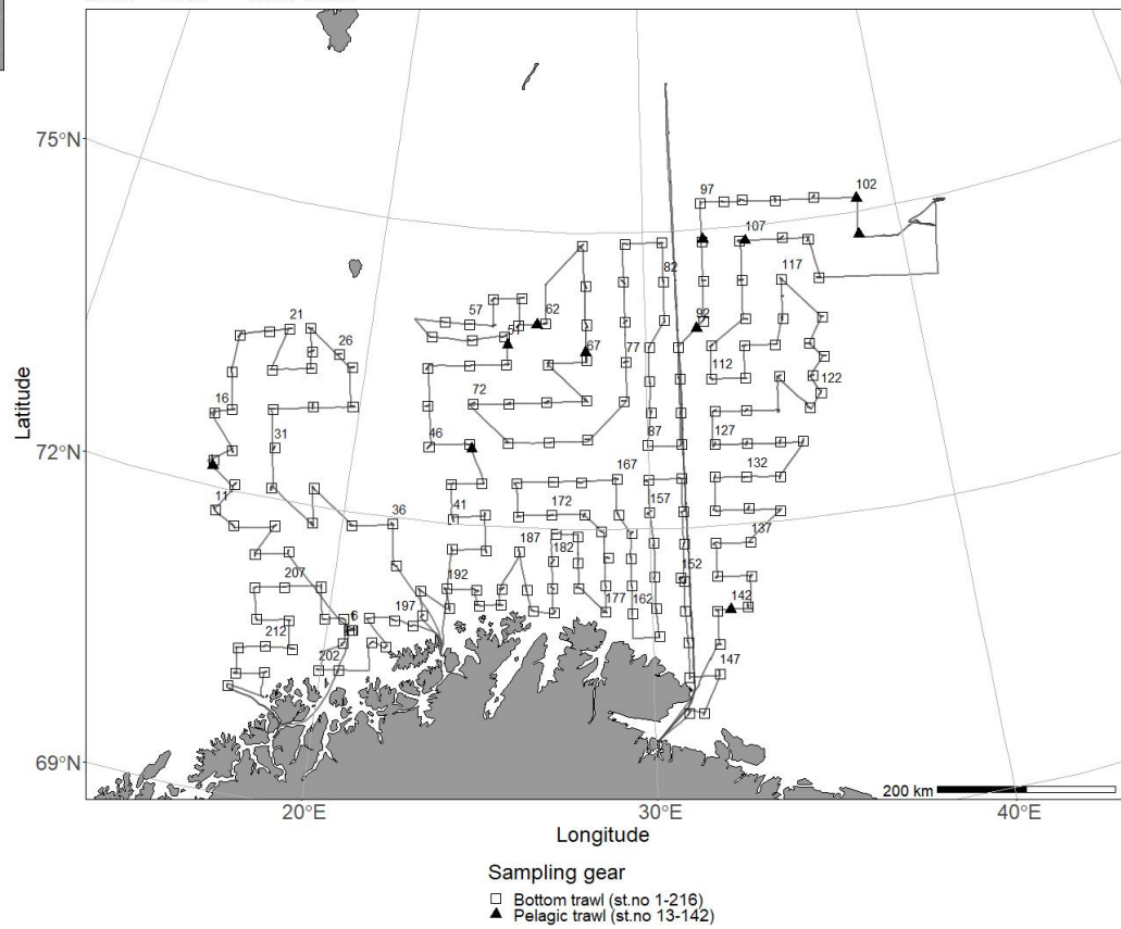
2022204 - Johan Hjort 27/01 - 14/03 - Trawl Chart
