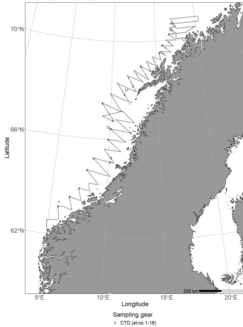
2022821 - Vendla 14/02 - 27/02 - CTD Chart
