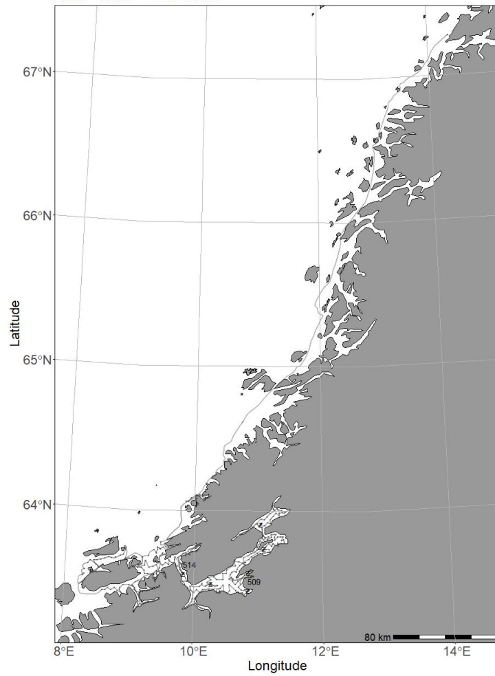
2022608 - Kristine Bonnevie 29/03 - 07/04 - CTD Chart
