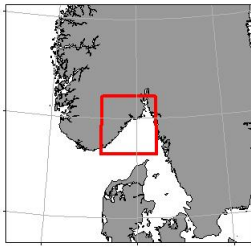
2022305 - G.M.Dannevig 20/04 - 27/04 - CTD Chart
