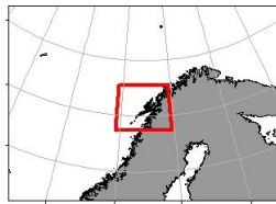
2022205 - Johan Hjort 20/03 - 09/04 - Trawl Chart
