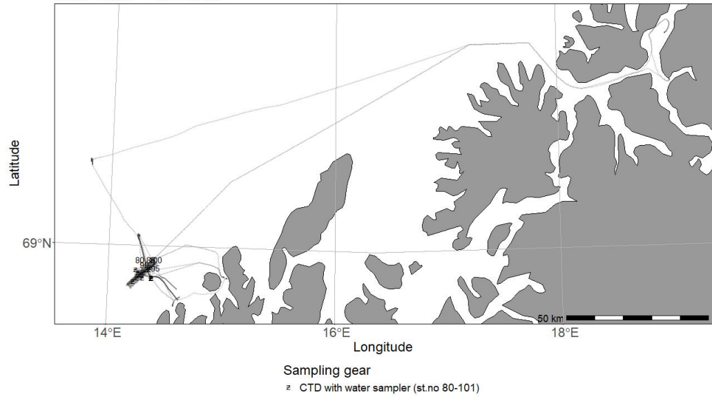
2022707 - Kronprins Haakon 01/06 - 16/06 - CTD Chart
