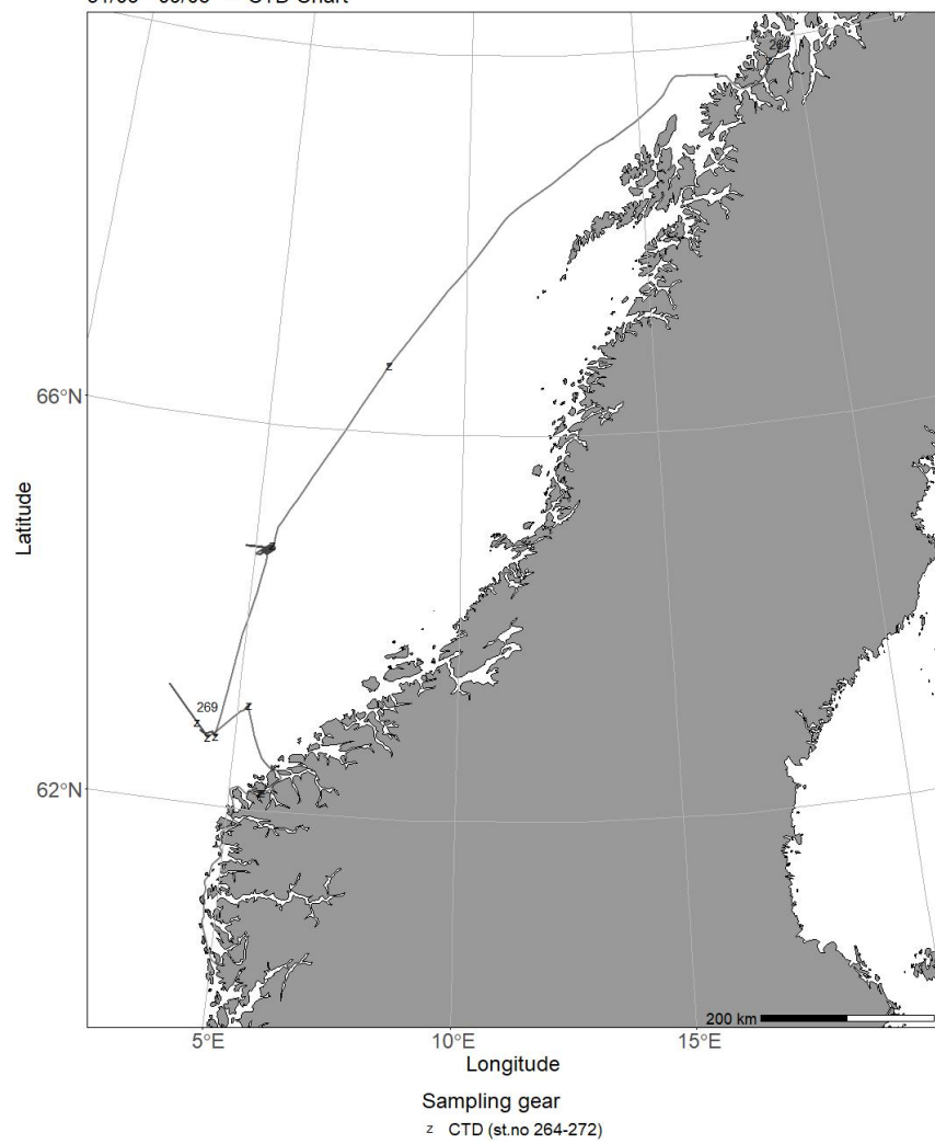
2022106 - G.O.Sars 31/05 - 09/06 - CTD Chart
