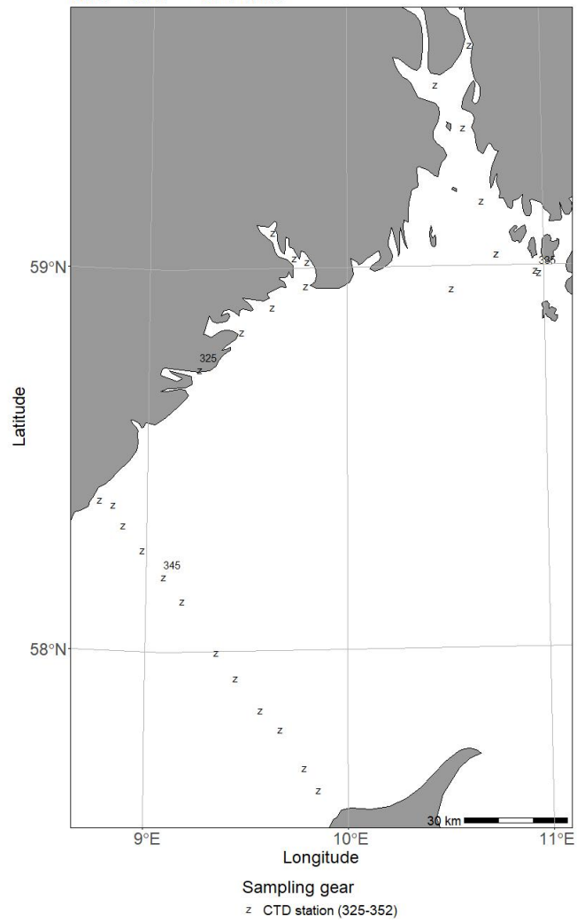
2022317 - G.M.Dannevig 08/11 - 13/11 - CTD Chart
