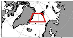
2022715 - Kronprins Haakon 24/08 - 07/09 - CTD Chart
