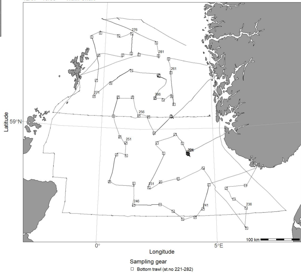
2022619 - Kristine Bonnevie 12/07 - 15/08 - Trawl Chart
