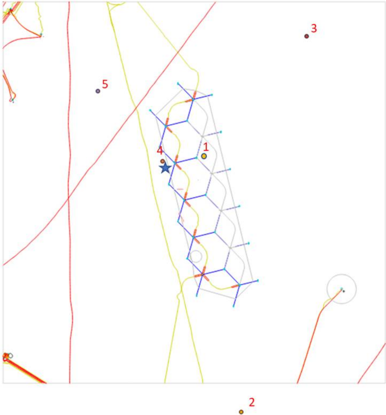
Figure 2. Map showing the positions where we deployed moorings at Hywind Tampen. The positions of the 5 ADCPs are marked with number 1 to 5, and the hydrophone marked with a blue star. The coordinates of the moorings are given in Table 2. Hywind Tampen windfarm: yellow line is cable, blue lines are anchor-chains. Turbines are positioned in the middle of three anchor-chains.
