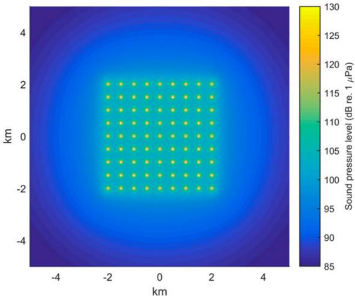
Figure 6. Operational noise for a 9 x 9 turbine offshore wind farm and park layout is given as [1] (Tougaard et al 2020)
