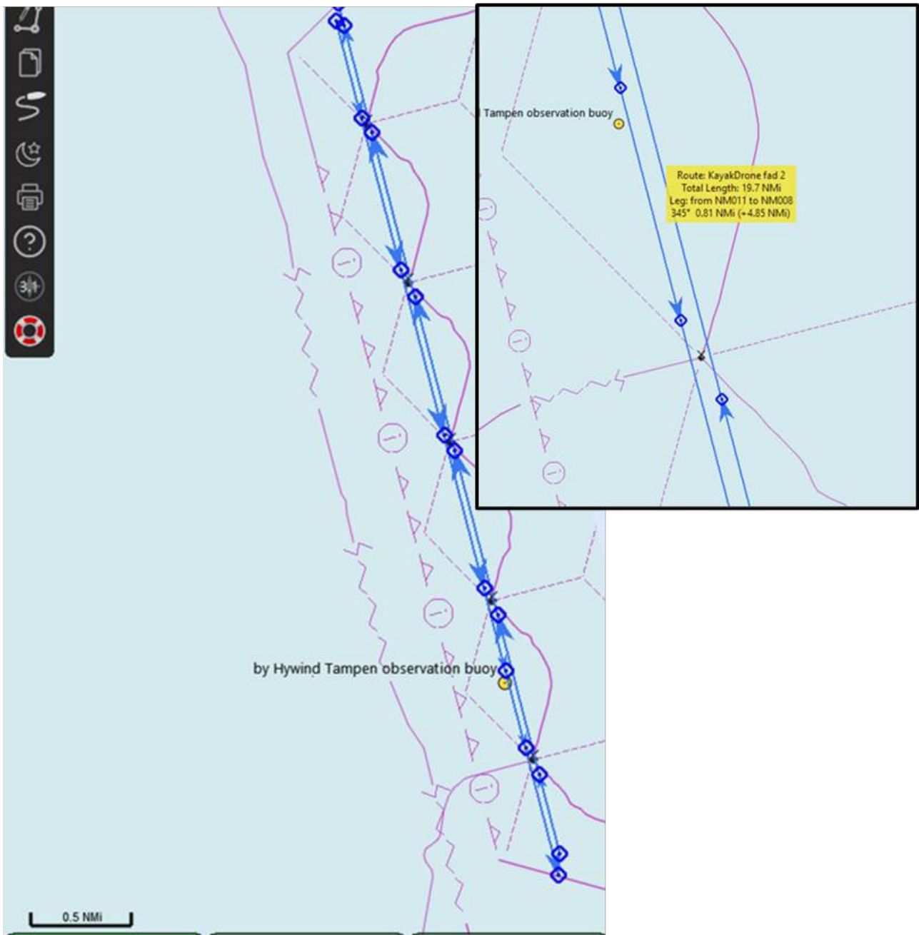
Figure 18. The KayakDrone's acoustic transect, survey design. Where the KayakDrone is to move between and passe by turbine: HY07, HY08, HY09, HY10, and HY11 all standing in one strait line. To the right: A close-up view of the KayakDrone's acoustic transect of the survey design. Blue circles are waypoint where the KayakDrone is repositioning related to the given coordinates in the transect.
