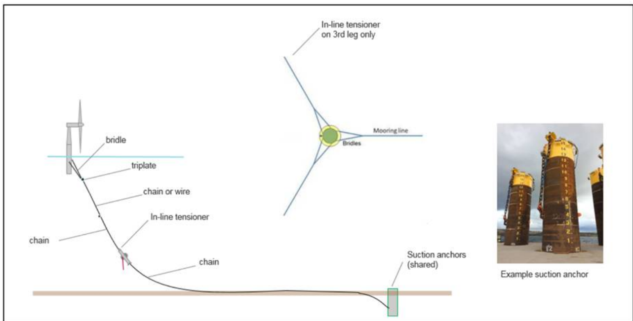
Figure 1: Illustration of anchoring of Hywind Tampen turbine copied from Equinor report: Hywind Tampen PUD del II – Konsekvensutredning 2019.
