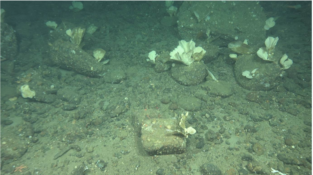
Figure 7 Hard bottom sponge garden at R3193 VL3274
