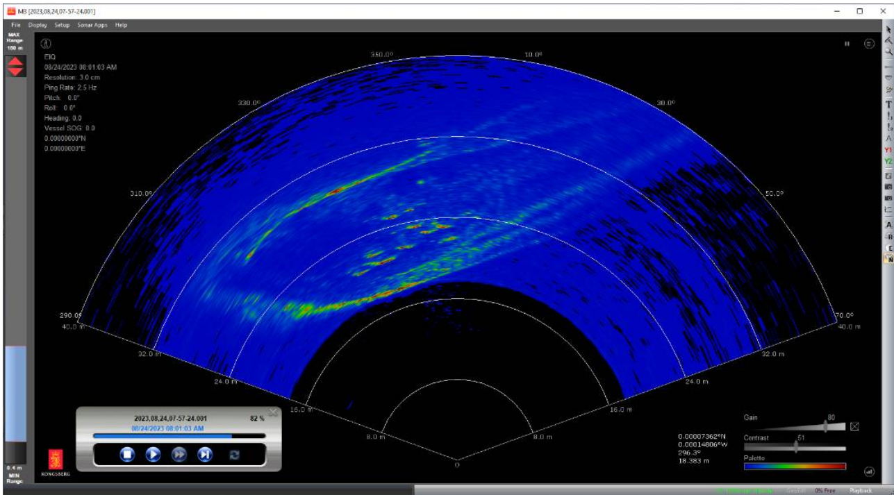
Figure 12: Screen dump from M3 sonar on 24.08.23 of the transfer cage with BFT from Cast 2. The group of BFT is observed in the center of the image as individually defined oval shape targets of color between green and orange. The two net walls of the transfer cage are shown as parallel lines mostly of light green and yellow. Transducer located ca. 18 m from net wall, sampling range of 40 m.
