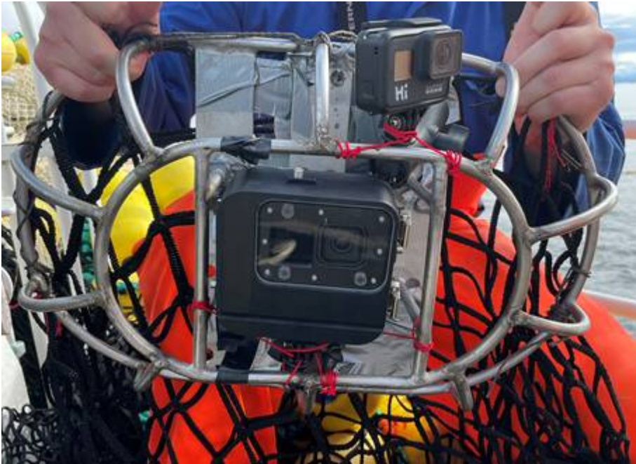
Figure 6: Steel frame with GoPro cameras fixed to the inside of the netting in the channel.
