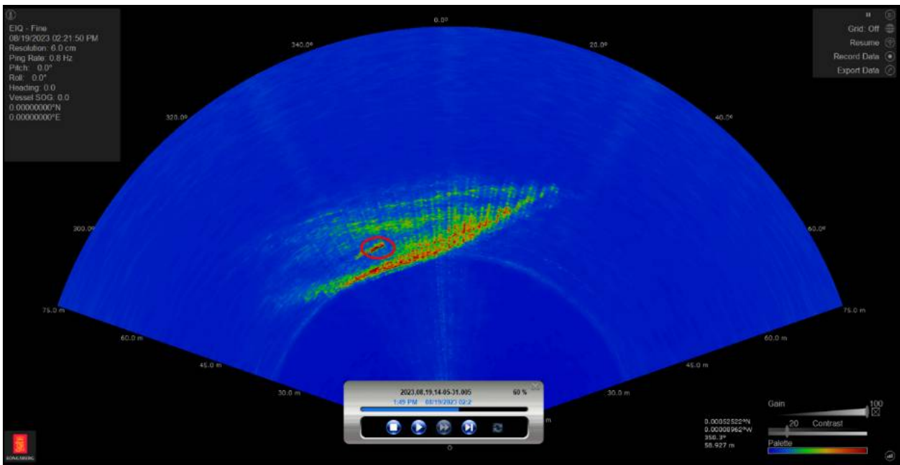
Figure 10: Screen dump from M3 sonar on 19.08.23 with a range of 75 m using EIQ-fine (Enhanced Image Quality) data acquisition mode. The single BFT is indicated with the red circle, the rest of the backscatter (green to orange) corresponds to the transfer cage. Data collected ca . 30 m away from net wall, with a sampling range of 75 m.
