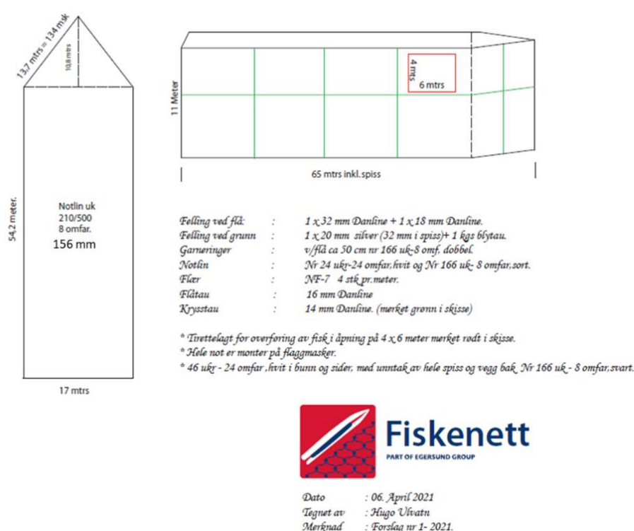
Figure 5: Construction of the transfer cage (left) and aerial view of the transfer cage while towing (right).
