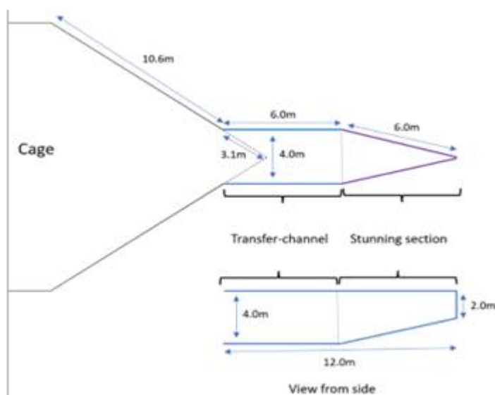
Figure 8: Schematic of the transfer (blue) and stunning channel (purple) attached at the lower end of the transfer cage. Below: side view of the transfer and stunning channel with approximate dimensions.
