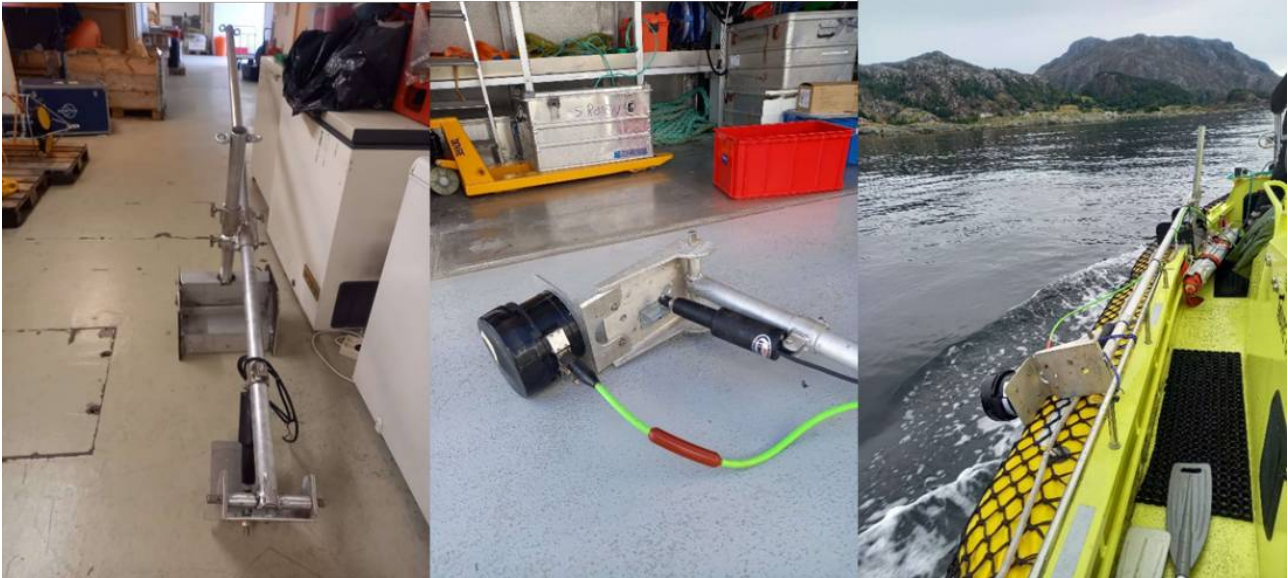
Figure 3: Pole for mounting the M3 sonar. Left: the whole pole with attachment points, including the system to allow retrieval from the water when moving and deployment into the water when acoustic sampling is underway. Middle: M3 transducer mounted to the end of the pole with a hydraulic arm to allow tilting. Right: pole mounted to skiff before deployment.
