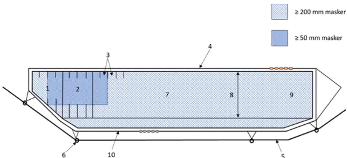
Figure 4: Schematic view of the seine with small mesh panel.
