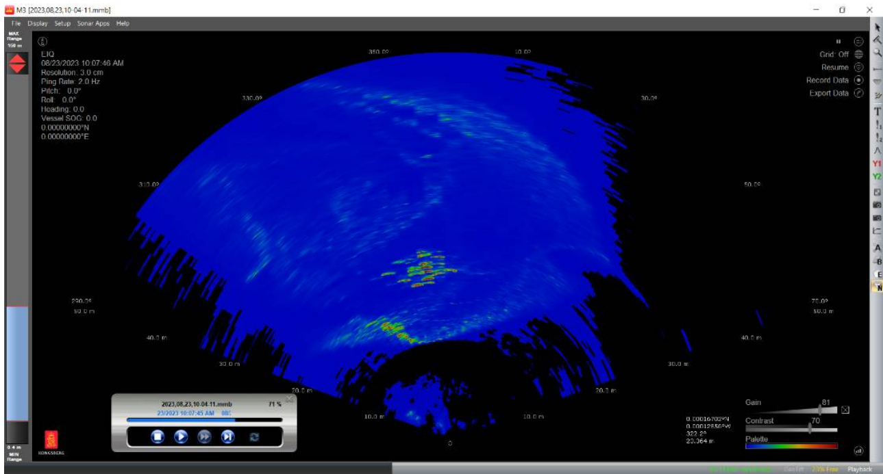
Figure 11: Screen dump from M3 sonar on 23.08.23 during Cast 2. The group of BFT is observed in the center of the image as individually defined oval shaped targets of color between green and orange. Light green and yellow elongated targets correspond to echoes from the purse seine net. Transducer located ca. 15 m from net wall, sampling range of 50 m.
