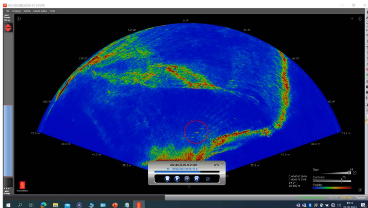
Figure 13. Screen dump from M3 sonar on 26.08.23 from inside the purse seine from Cast 3. The three BFT are circled in red. The larger and elongated scatters correspond to the purse seine net. Transducer located ca. 10 m from net wall with a sampling range of 75 m.
