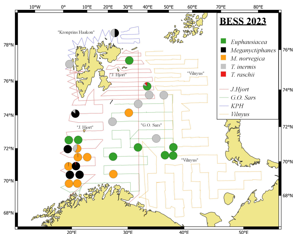
Figure 5.3.1.3. Krill species distribution, based on pelagic trawl catches covering 0-60 m, in the Barents Sea in August-October 2023.
