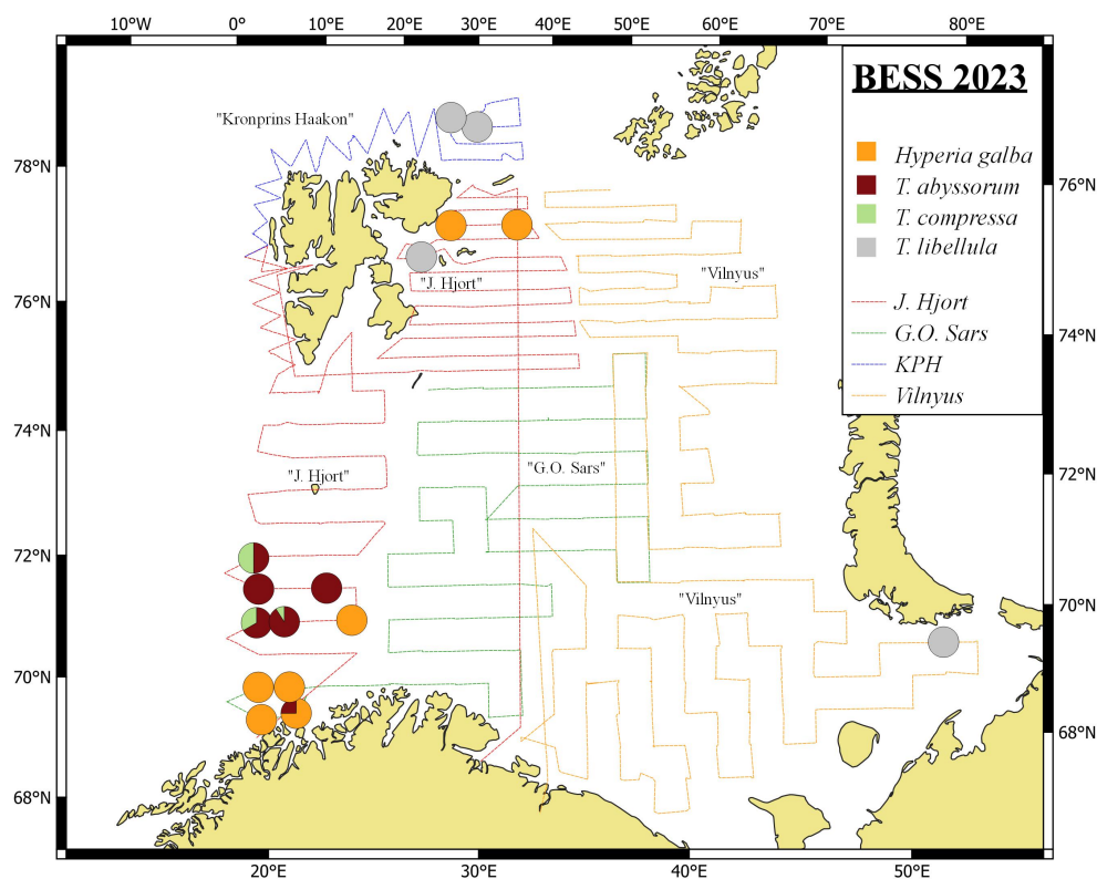
Figure 5.3.2.2. Distribution of pelagic amphipod species, based on pelagic trawl catches covering 0-60 m, in the Barents Sea in August-October 2023.
