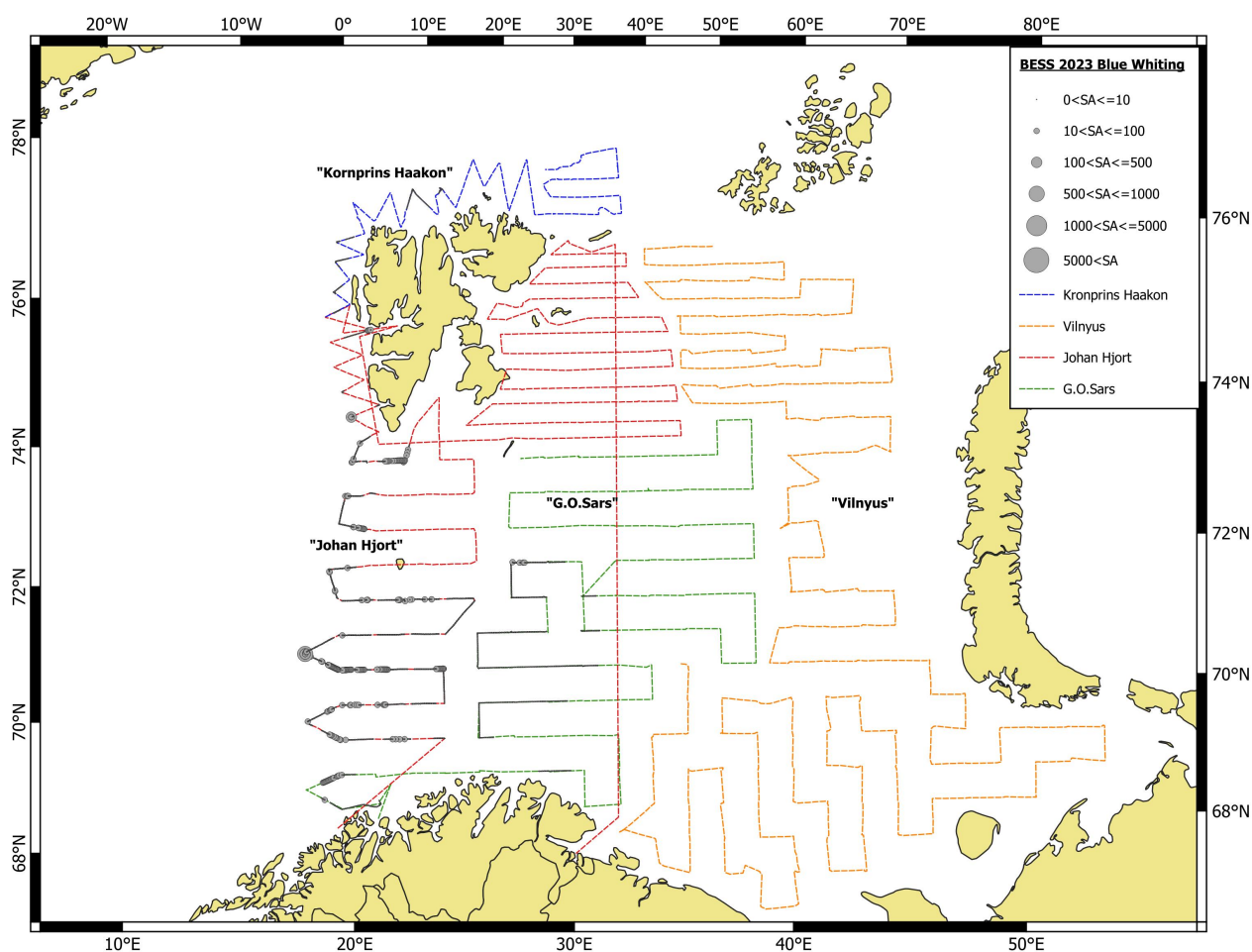
Figure 7.4.1.1. Geographical distribution of blue whiting in autumn 2023 based on acoustic recordings. Circle sizes correspond to NASC values ( m^2/nmi^2 ) per nautical mile.
