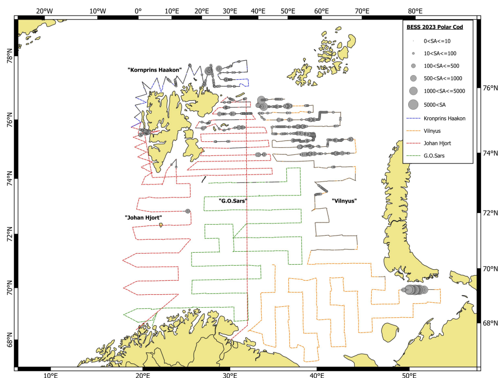
Figure 7.2.1.1 Geographical distribution of polar cod in autumn 2023 based on acoustic data. Circle sizes correspond to NASC values ( \text{m}^2/\text{nm}^2 ) per nautical mile.
