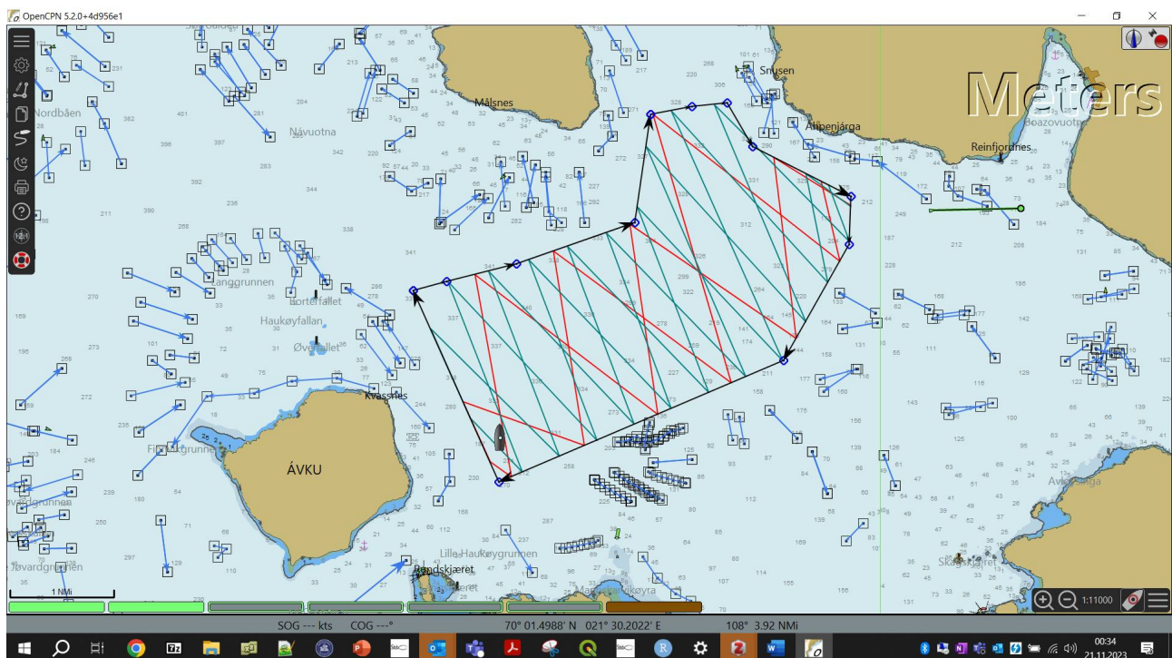
Figure 20 USV Frigg versus RV G.O. Sars experiment A. Planned transects of USV Frigg is marked as red, and the transects of G.O. Sars are depicted in green.
