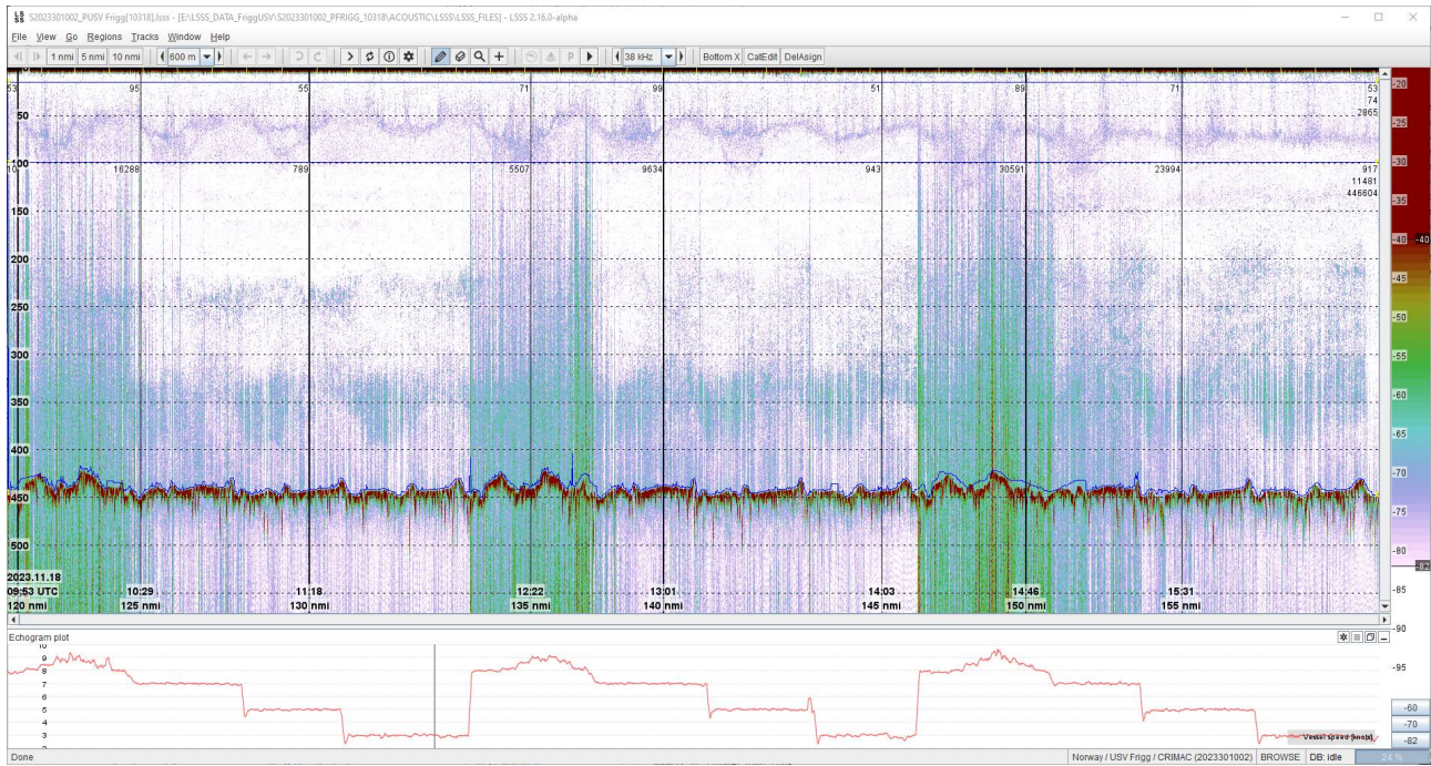
Figure 12 . Echogram from USV Frigg taken from the Austerhola octagon in BF4. Note the vertical stripes indicating loss of acoustic backscatter caused by bubble attenuation. The increased noise cause by increased speed is seen as the green "columns" in the echogram.
