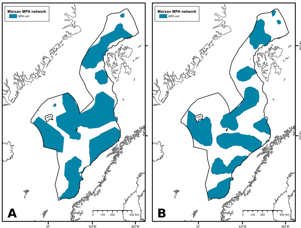
Figure 3. Selection of two different scenarios of MPA networks protecting A (left): 50% and B (right): 40% of the total study area.
