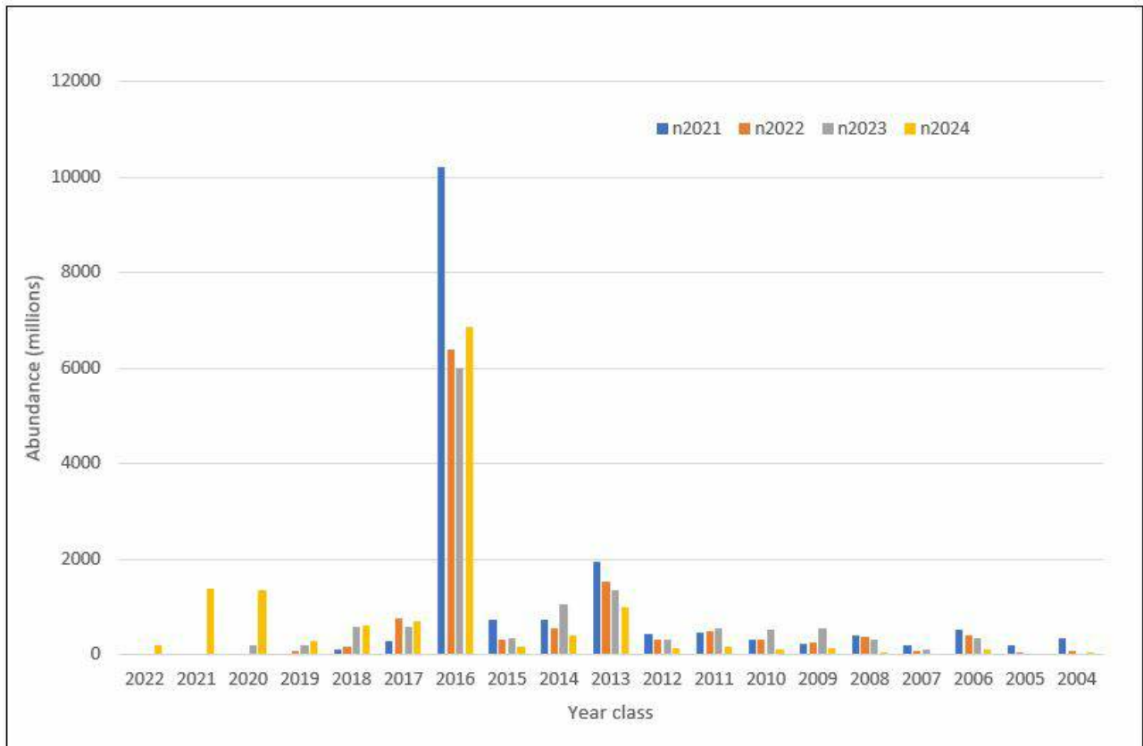
Figure 6. Abundance by year class estimated during the Norwegian spring-spawning herring spawning surveys 2021-2024 (mean of 1000 bootstrap replicates). Legend: Separate color for each survey year.
