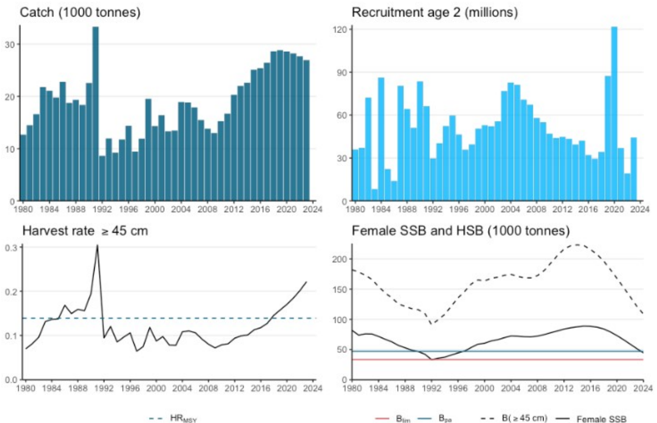
Figure 1. Greenland halibut in ICES subareas 1 and 2 (Northeast Arctic). From top left to bottom right: catches, recruitment at age 2, harvest rate for fish \geq 45 cm with estimated HR_{MSY} , and female SSB as well as HSB (harvestable stock biomass defined as \geq 45 cm fish). The biomass reference points relate to female SSB.
