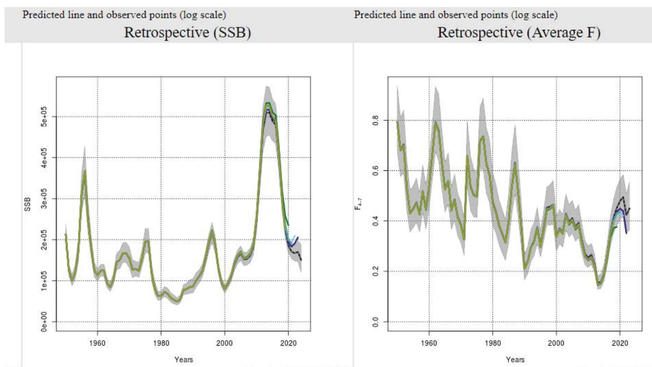
Figure 4.3. Northeast Arctic haddock. 5 year retrospective plots of Recruitment (top left), catch (top middle) and TSB (top right), SSB (bottom left), and fishing mortality TSB (bottom right) for years 1950–2024 (2023 catches and F ) (SAM with 95% confidence intervals).
