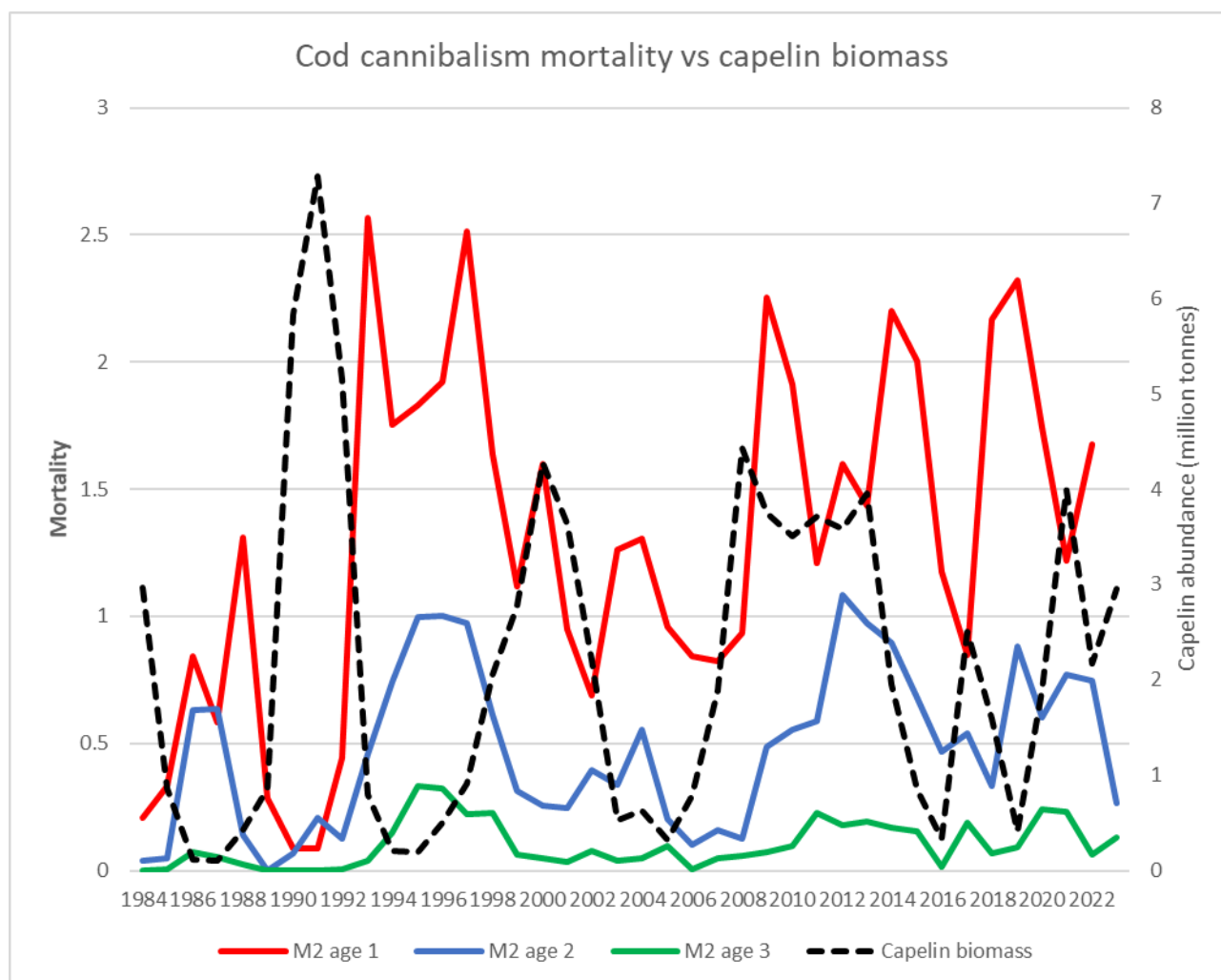
Figure 3.3. NEA cod cannibalism mortality vs. capelin abundance.
