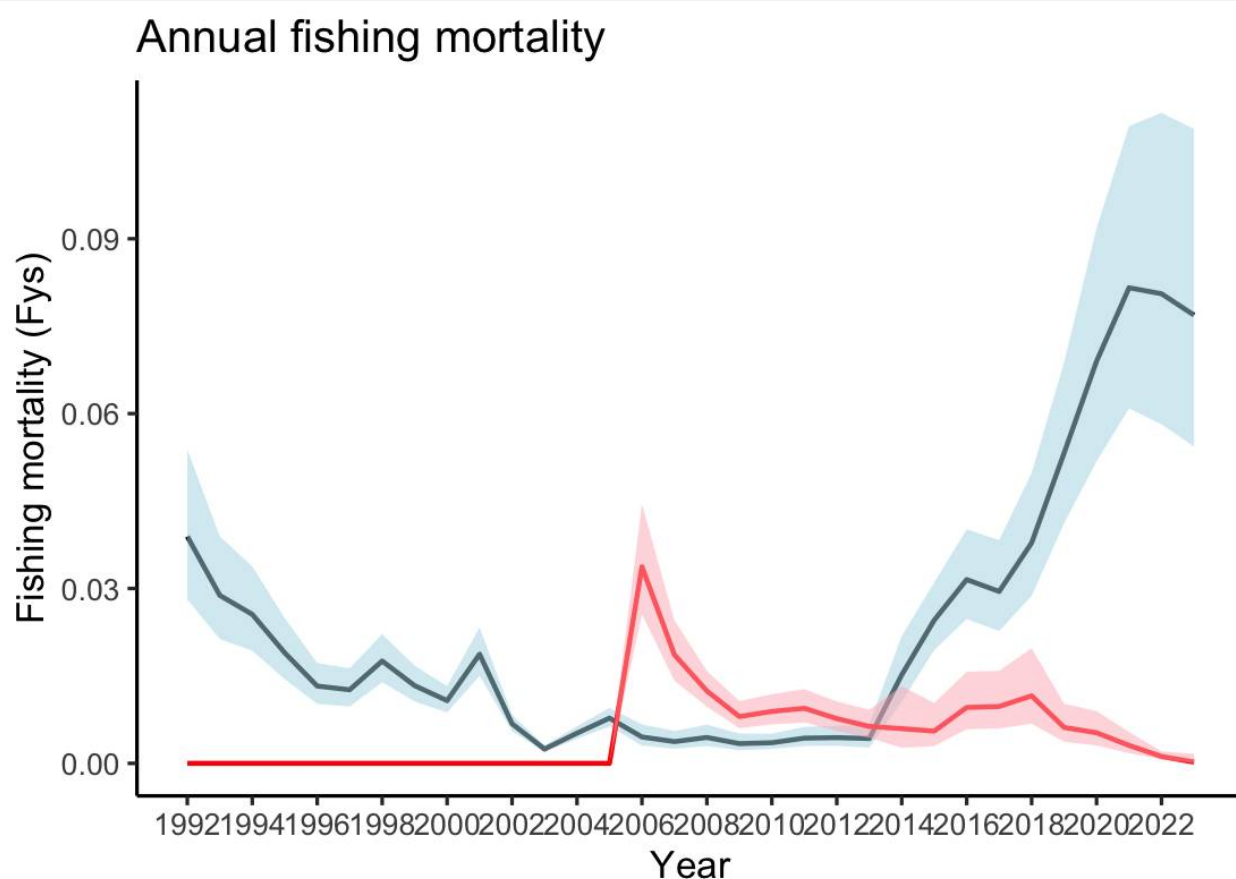
Figure 6.18. S. mentella in subareas 1 and 2. Results from the statistical catch-at-age assessment run showing the estimated recruitment-at-age 2 spawning-stock biomass from 1992 to 2023 and annual fishing mortality coefficients by year ( F_y ) from the demersal (blue) and pelagic (red) fleets. Error bars (top) and the colored envelope (bottom) indicate 95% confidence limits.
