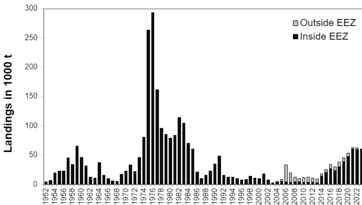
Figure 6.1. S. mentella in subareas 1 and 2. Total international landings 1952–2023 (thousand tonnes).
