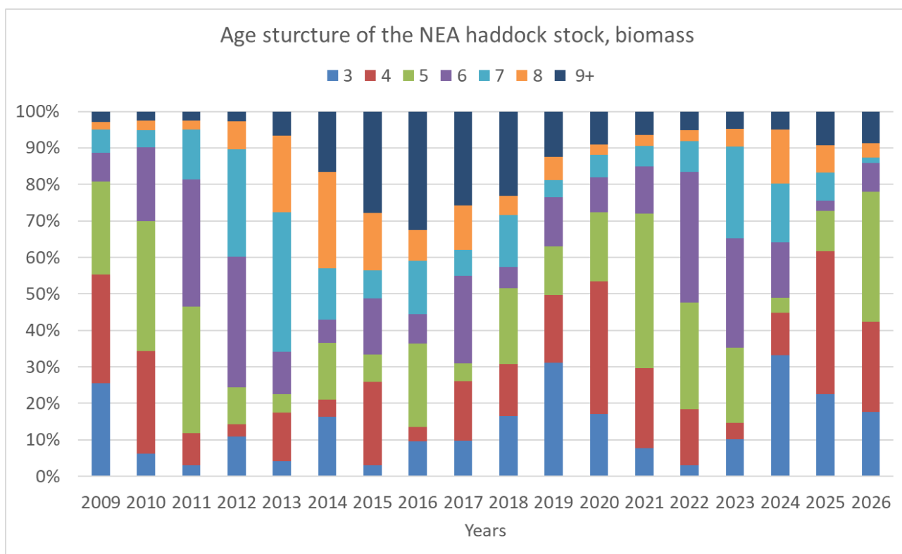
Figure 4.9. Age structure from assessment (2009-2024) and prediction (2025-2026).
