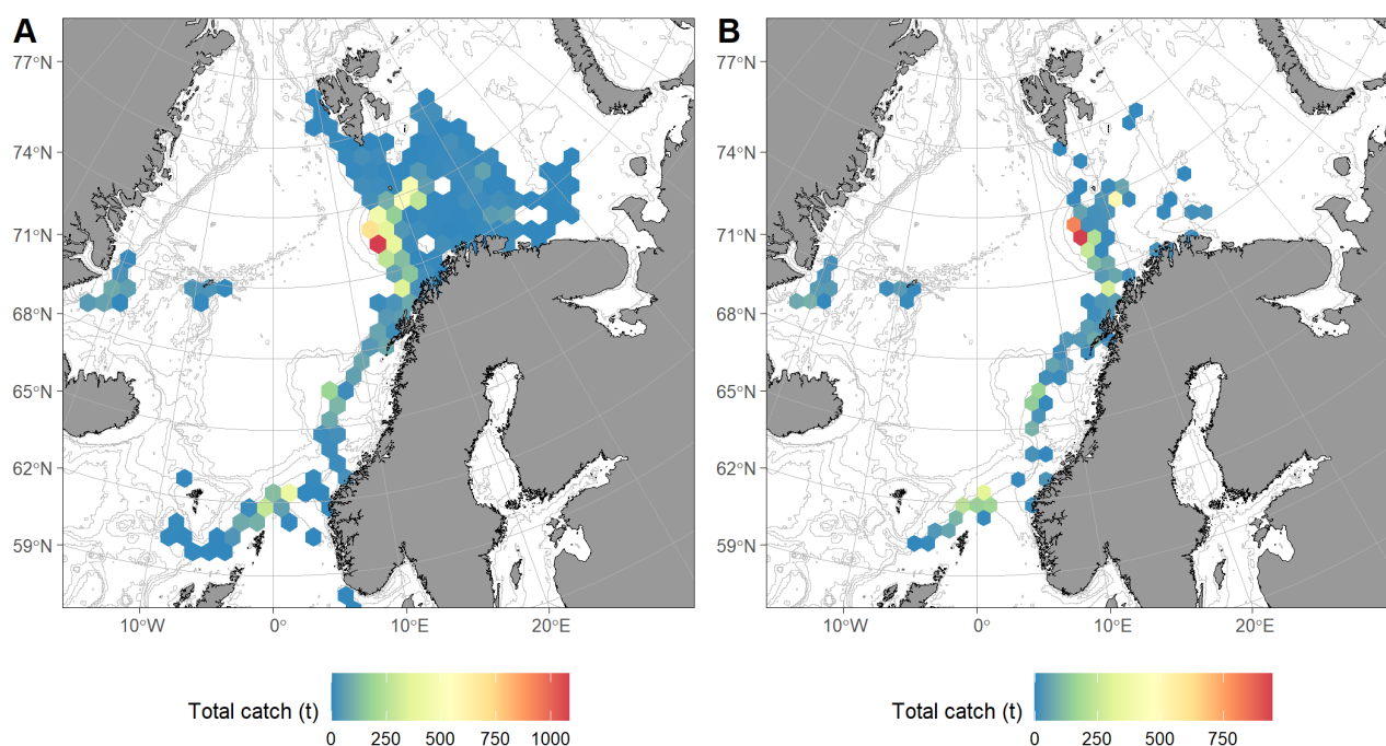
Figure 8.2. Spatial distribution of Greenland halibut catches in 2023 according to Norwegian electronic logbooks, in all registered fisheries including bycatch (A), and catches where Greenland halibut make more than 50% of the total catches (B).
