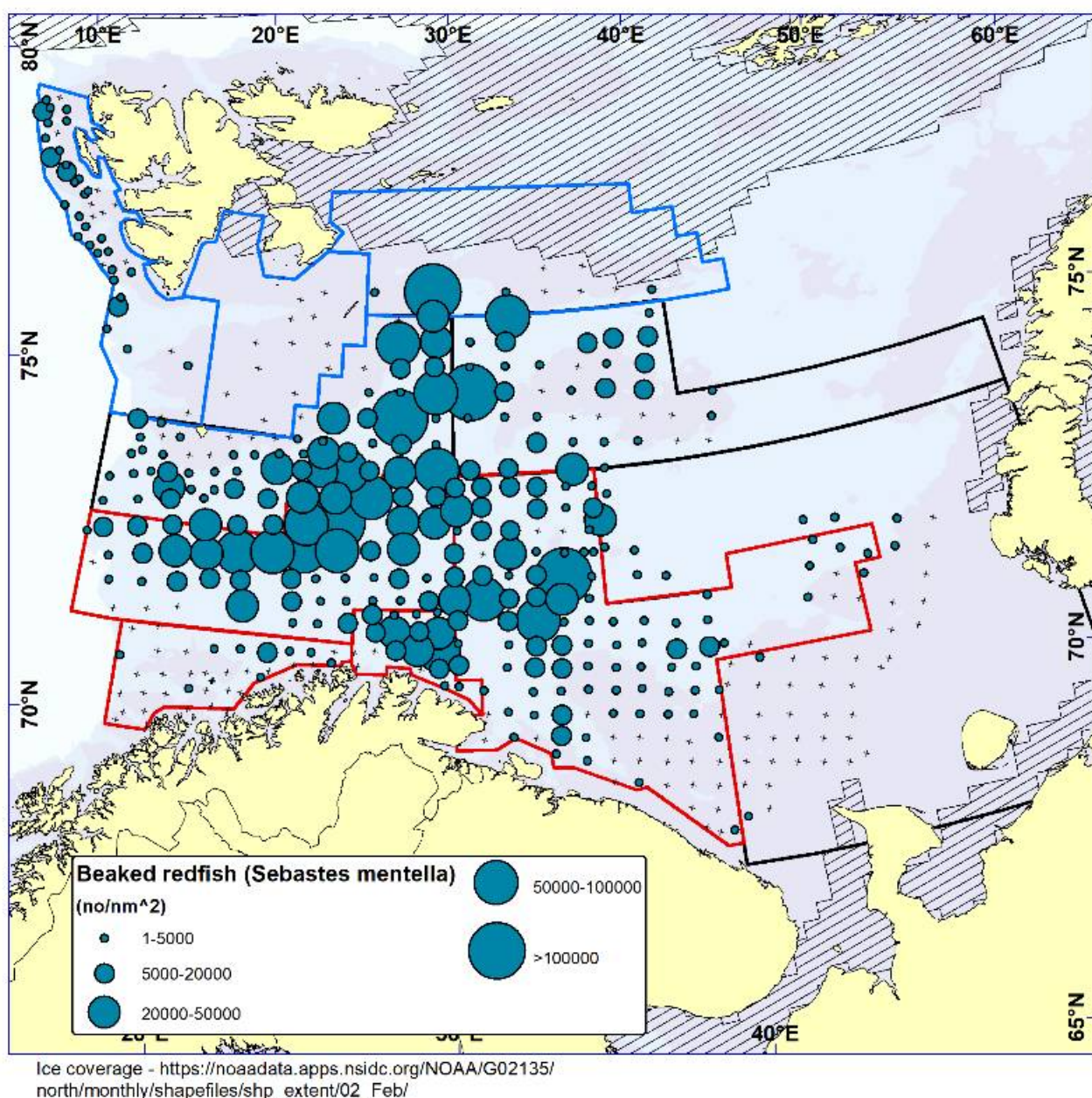
Figure 6.12. S. mentella in subareas 1 and 2. Abundance indices for individual trawl stations during the ecosystem survey in autumn 2023 (top) and winter survey 2023 (bottom).
