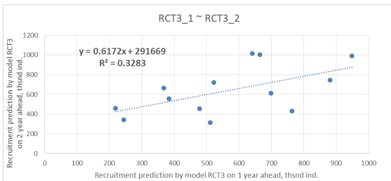
Figure 3. Correlation between retrospective recruitment RCT3 forecasts for 1 and 2 years ahead.
