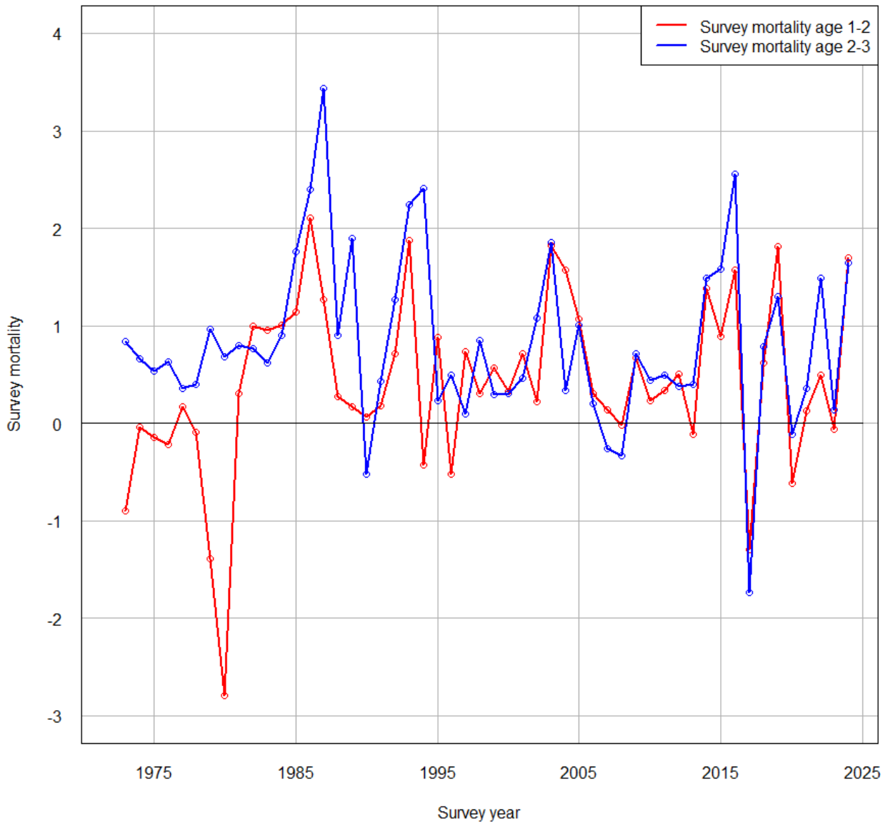
Figure A3. Survey mortality by survey year. Survey mortality is calculated as -\log((N \text{ age } (a+1) \text{ in year } (y+1) + \text{catch immatures of age } a \text{ in year } y \text{ and year } (y+1))/N \text{ immatures age } a \text{ in year } y) . Capelin >14.0 cm are assumed to be maturing.
